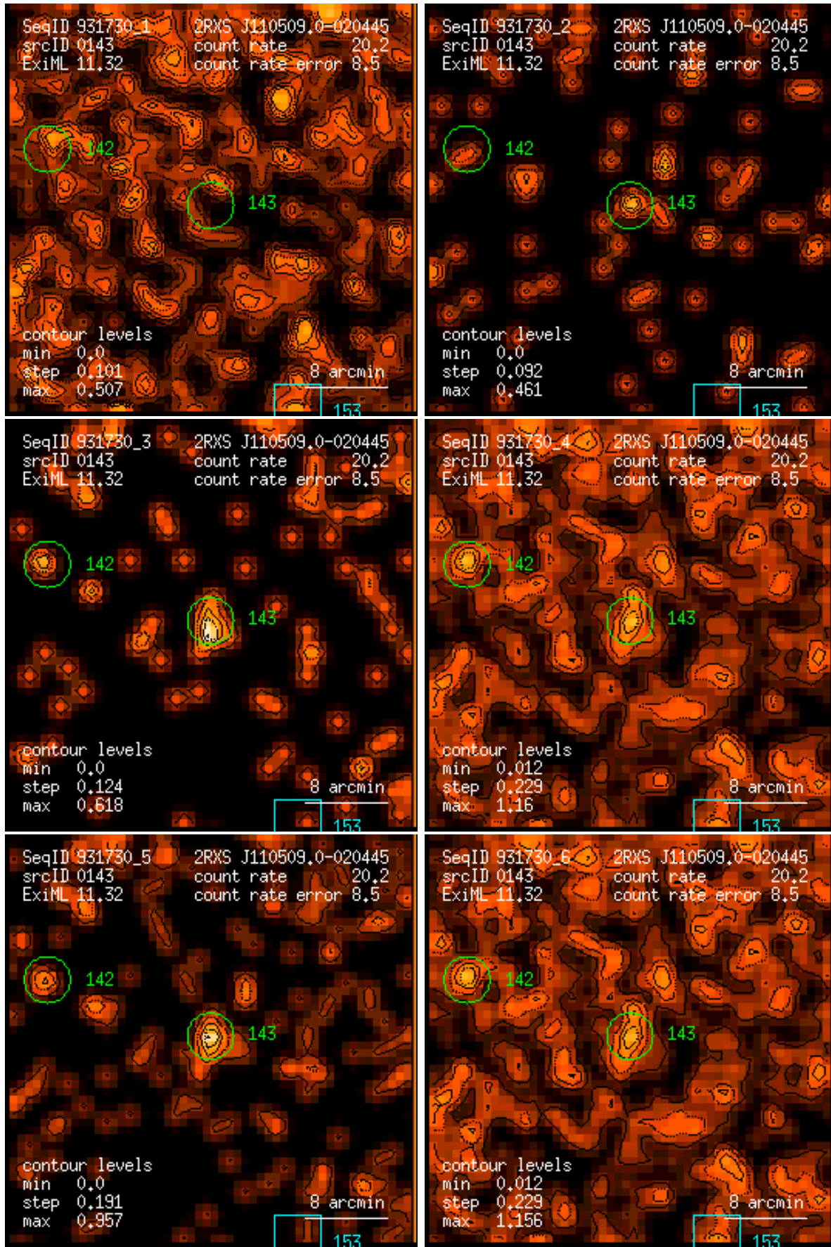
Figure 143: RASS 931730: detection 0143: band rate images, Gaussian filter: (1) PSPC channels 11 – 41, (2) 52 – 90, (3) 91 – 201, (4) 11 – 235, (5) 52 – 201, (6) 11 – 201. Broad band rates in counts/ks. Band rate contour levels in counts/ks/arcmin 2 .
