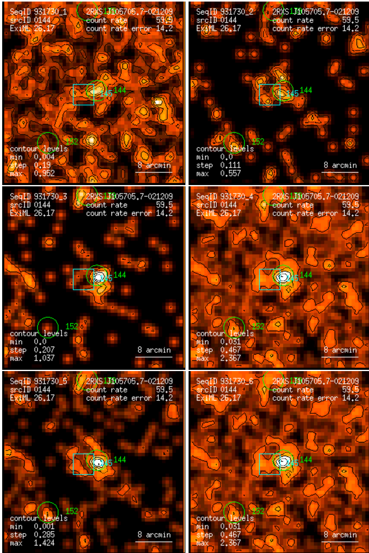
Figure 144: RASS 931730: detection 0144: band rate images, Gaussian filter: (1) PSPC channels 11 – 41, (2) 52 – 90, (3) 91 – 201, (4) 11 – 235, (5) 52 – 201, (6) 11 – 201. Broad band rates in counts/ks. Band rate contour levels in counts/ks/arcmin 2 .
