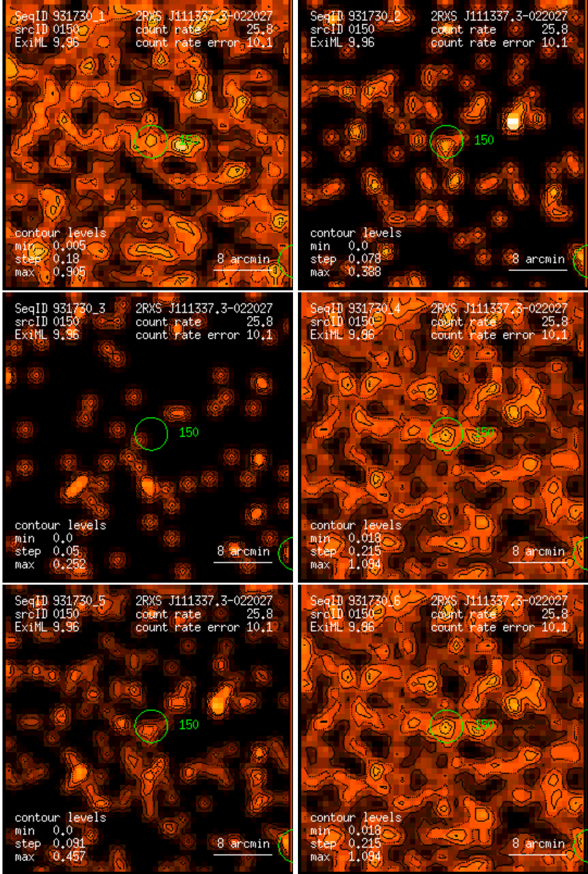
Figure 150: RASS 931730: detection 0150: band rate images, Gaussian filter: (1) PSPC channels 11 – 41, (2) 52 – 90, (3) 91 – 201, (4) 11 – 235, (5) 52 – 201, (6) 11 – 201. Broad band rates in counts/ks. Band rate contour levels in counts/ks/arcmin 2 .
