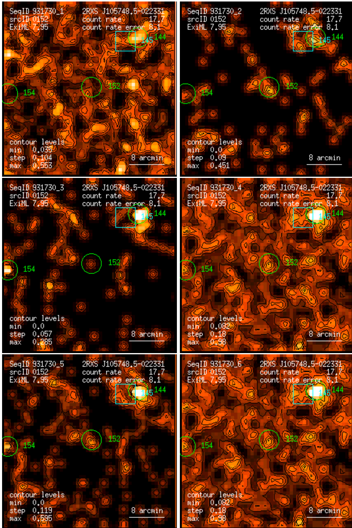
Figure 152: RASS 931730: detection 0152: band rate images, Gaussian filter: (1) PSPC channels 11 – 41, (2) 52 – 90, (3) 91 – 201, (4) 11 – 235, (5) 52 – 201, (6) 11 – 201. Broad band rates in counts/ks. Band rate contour levels in counts/ks/arcmin 2 .
