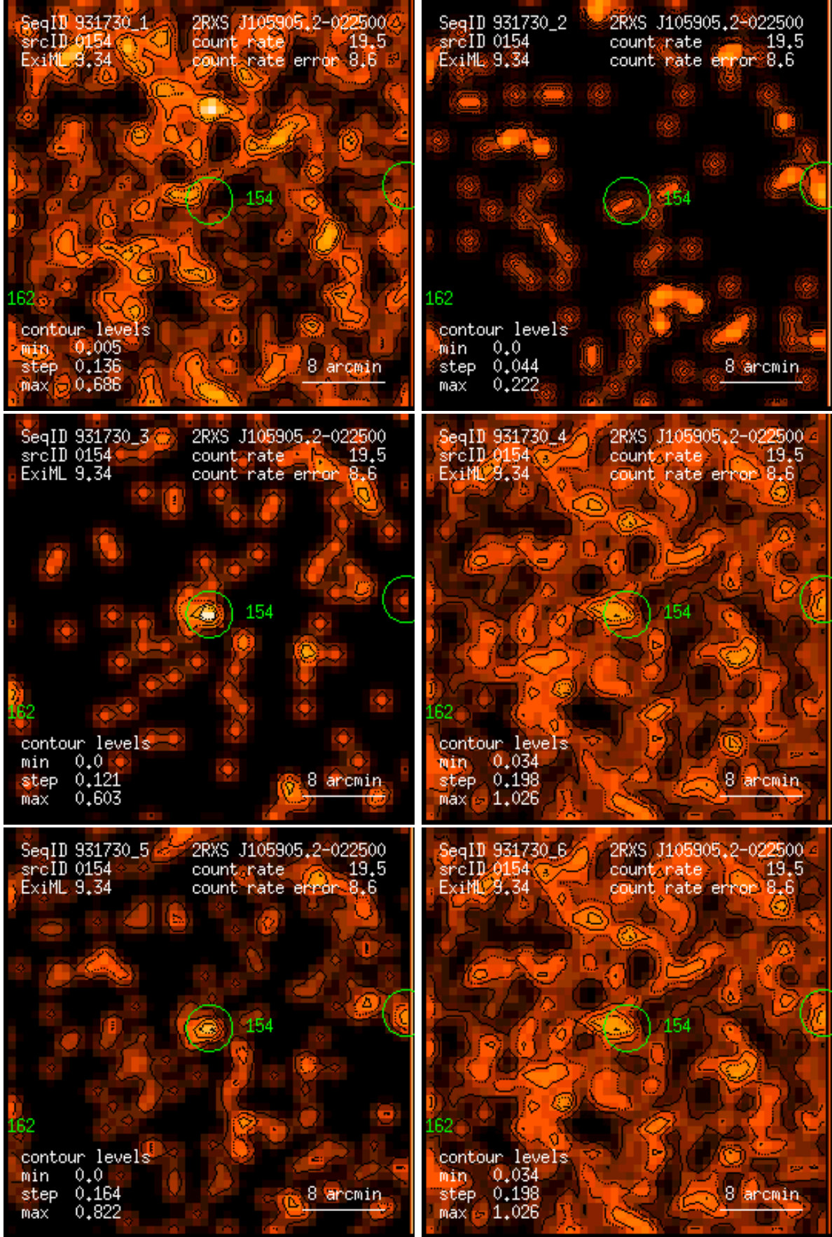
Figure 154: RASS 931730: detection 0154: band rate images, Gaussian filter: (1) PSPC channels 11 – 41, (2) 52 – 90, (3) 91 – 201, (4) 11 – 235, (5) 52 – 201, (6) 11 – 201. Broad band rates in counts/ks. Band rate contour levels in counts/ks/arcmin 2 .
