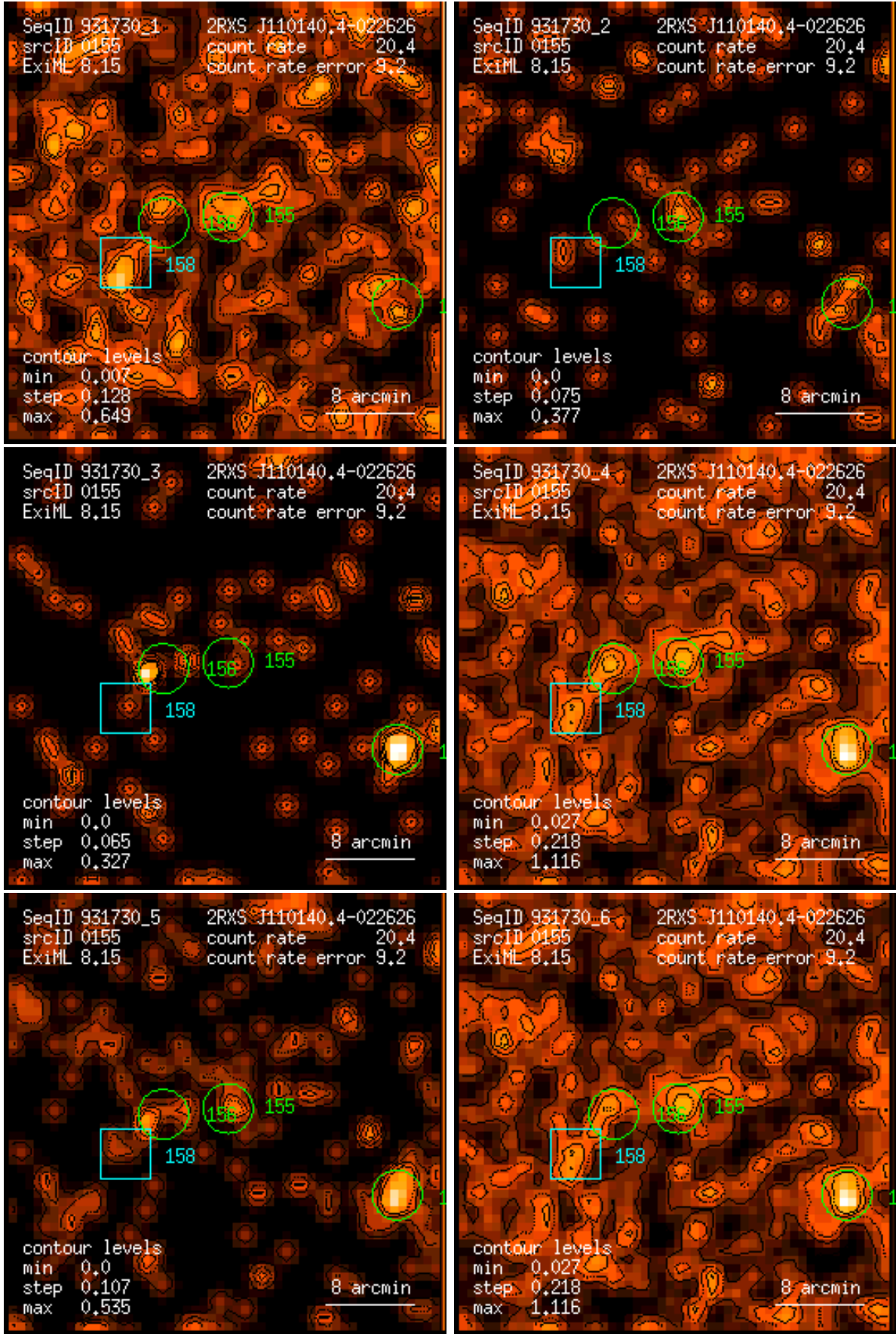
Figure 155: RASS 931730: detection 0155: band rate images, Gaussian filter: (1) PSPC channels 11 – 41, (2) 52 – 90, (3) 91 – 201, (4) 11 – 235, (5) 52 – 201, (6) 11 – 201. Broad band rates in counts/ks. Band rate contour levels in counts/ks/arcmin 2 .
