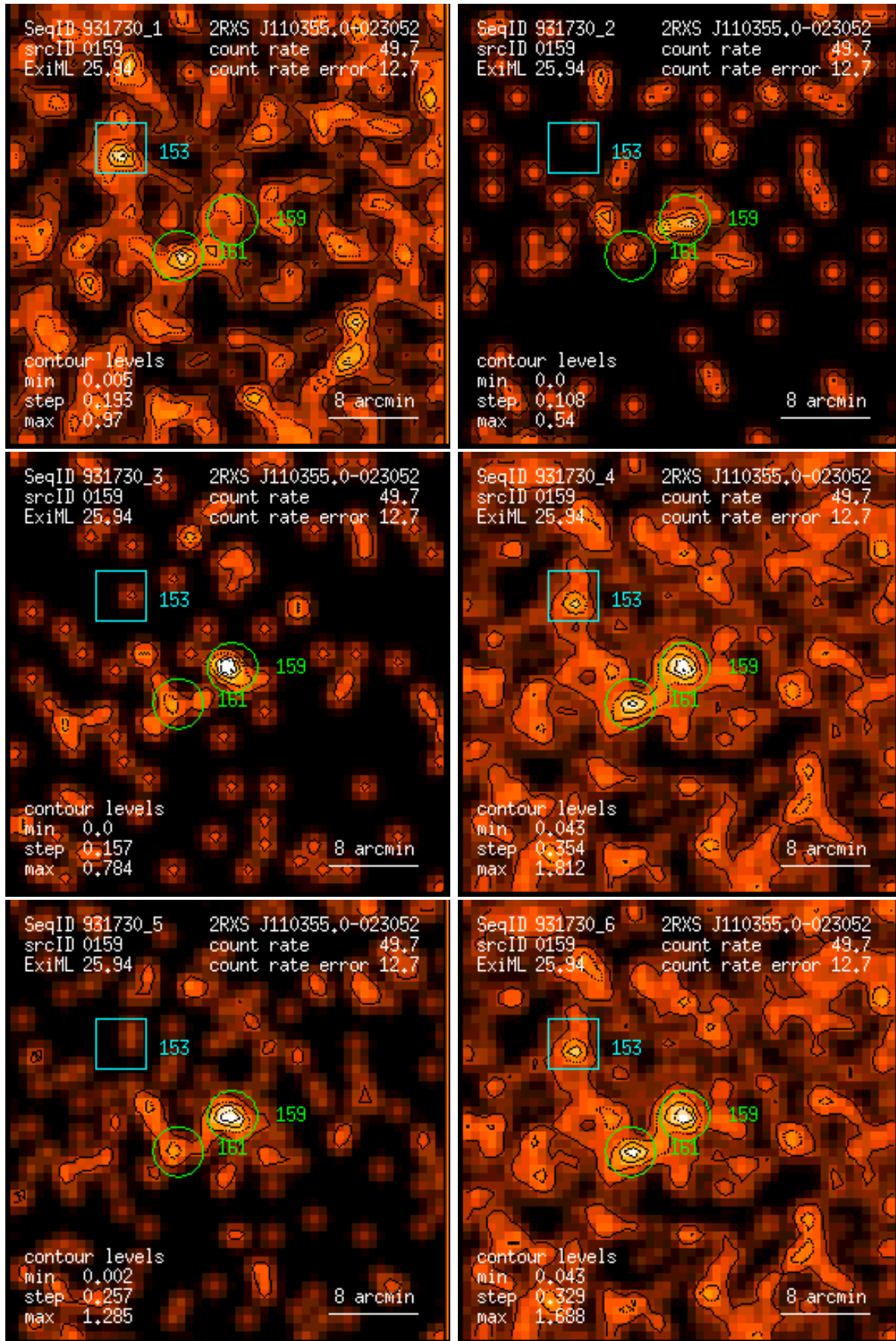
Figure 159: RASS 931730: detection 0159: band rate images, Gaussian filter: (1) PSPC channels 11 – 41, (2) 52 – 90, (3) 91 – 201, (4) 11 – 235, (5) 52 – 201, (6) 11 – 201. Broad band rates in counts/ks. Band rate contour levels in counts/ks/arcmin 2 .
