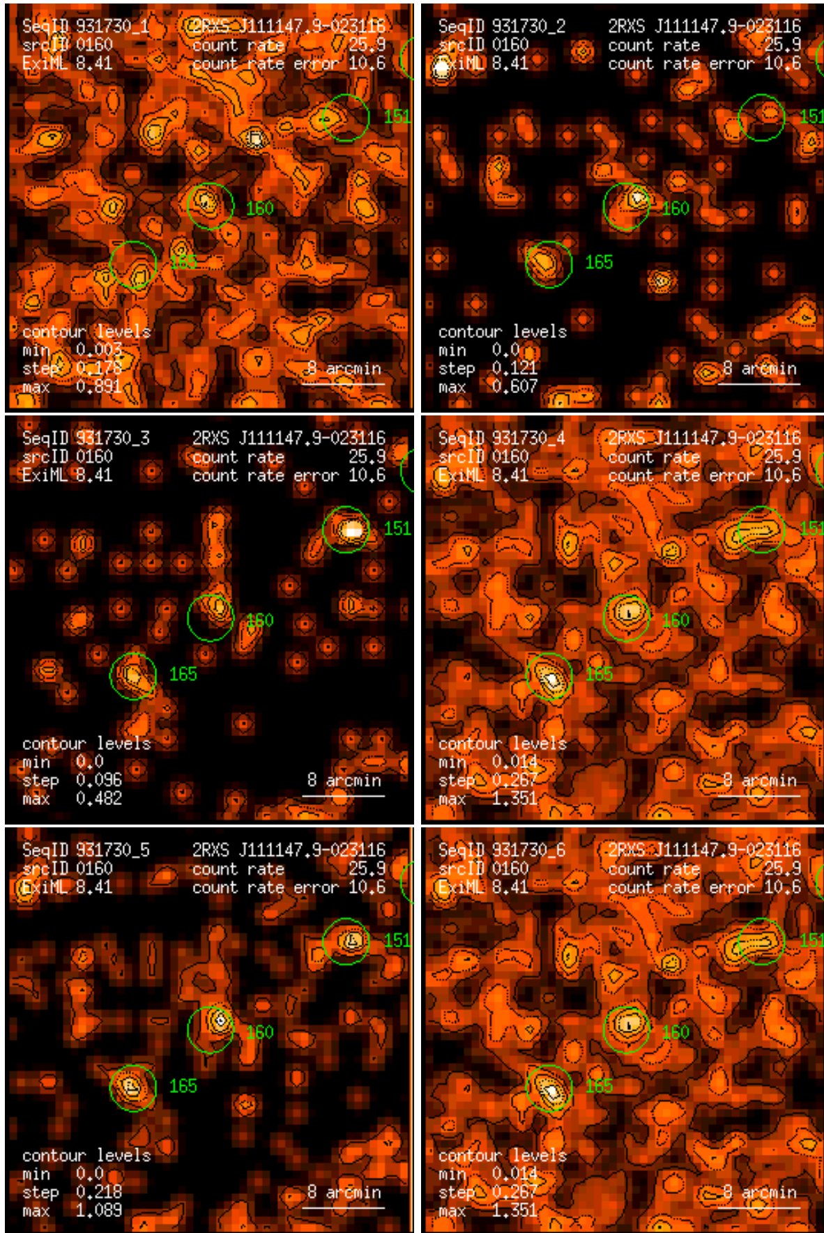
Figure 160: RASS 931730: detection 0160: band rate images, Gaussian filter: (1) PSPC channels 11 – 41, (2) 52 – 90, (3) 91 – 201, (4) 11 – 235, (5) 52 – 201, (6) 11 – 201. Broad band rates in counts/ks. Band rate contour levels in counts/ks/arcmin 2 .
