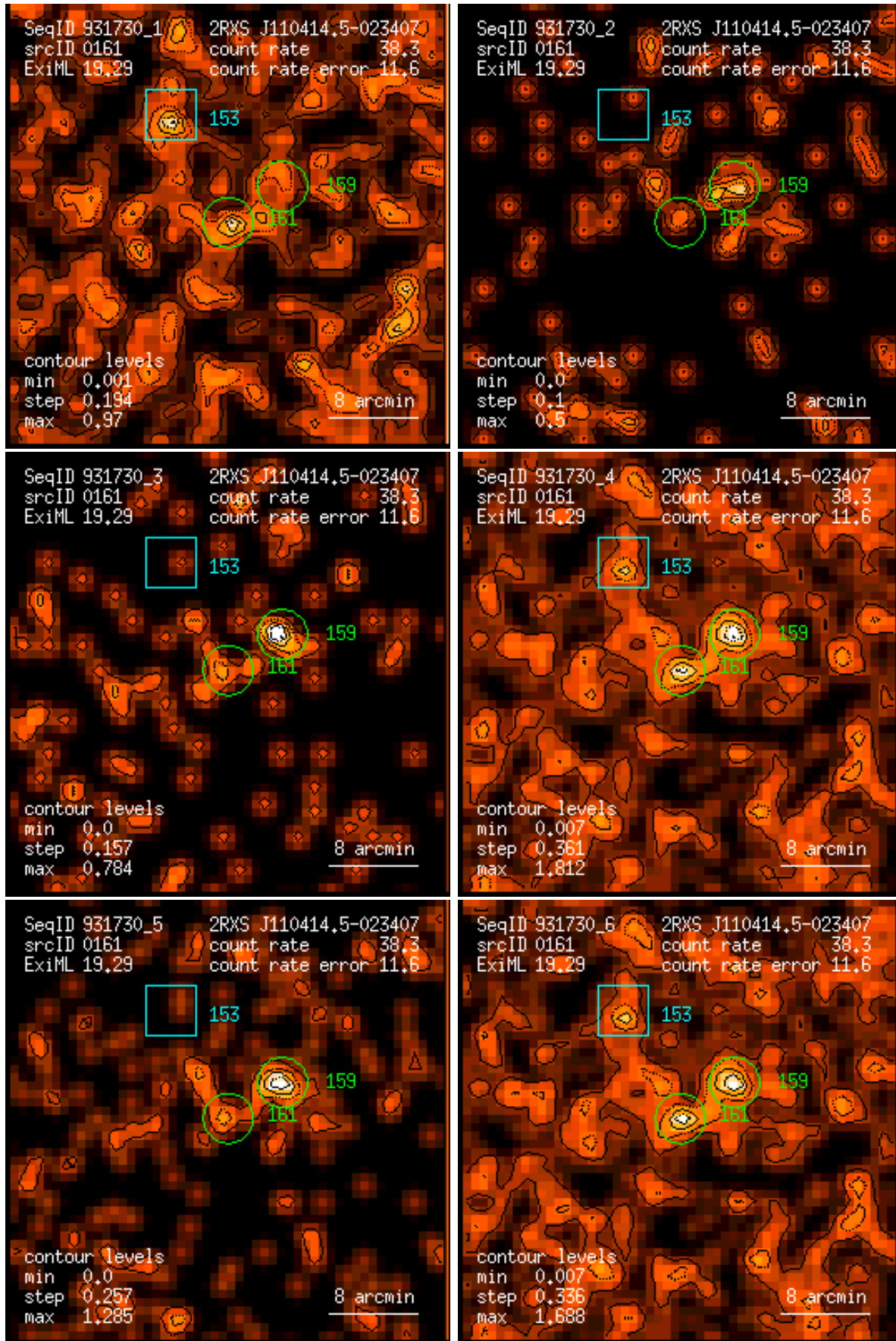
Figure 161: RASS 931730: detection 0161: band rate images, Gaussian filter: (1) PSPC channels 11 – 41, (2) 52 – 90, (3) 91 – 201, (4) 11 – 235, (5) 52 – 201, (6) 11 – 201. Broad band rates in counts/ks. Band rate contour levels in counts/ks/arcmin 2 .
