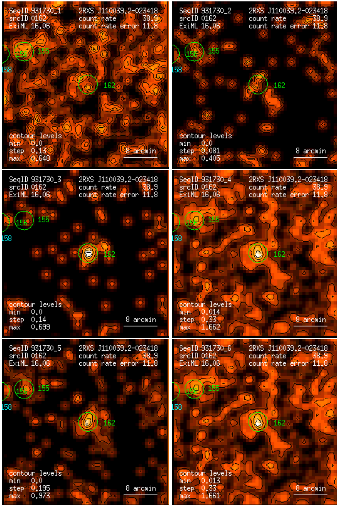
Figure 162: RASS 931730: detection 0162: band rate images, Gaussian filter: (1) PSPC channels 11 – 41, (2) 52 – 90, (3) 91 – 201, (4) 11 – 235, (5) 52 – 201, (6) 11 – 201. Broad band rates in counts/ks. Band rate contour levels in counts/ks/arcmin 2 .
