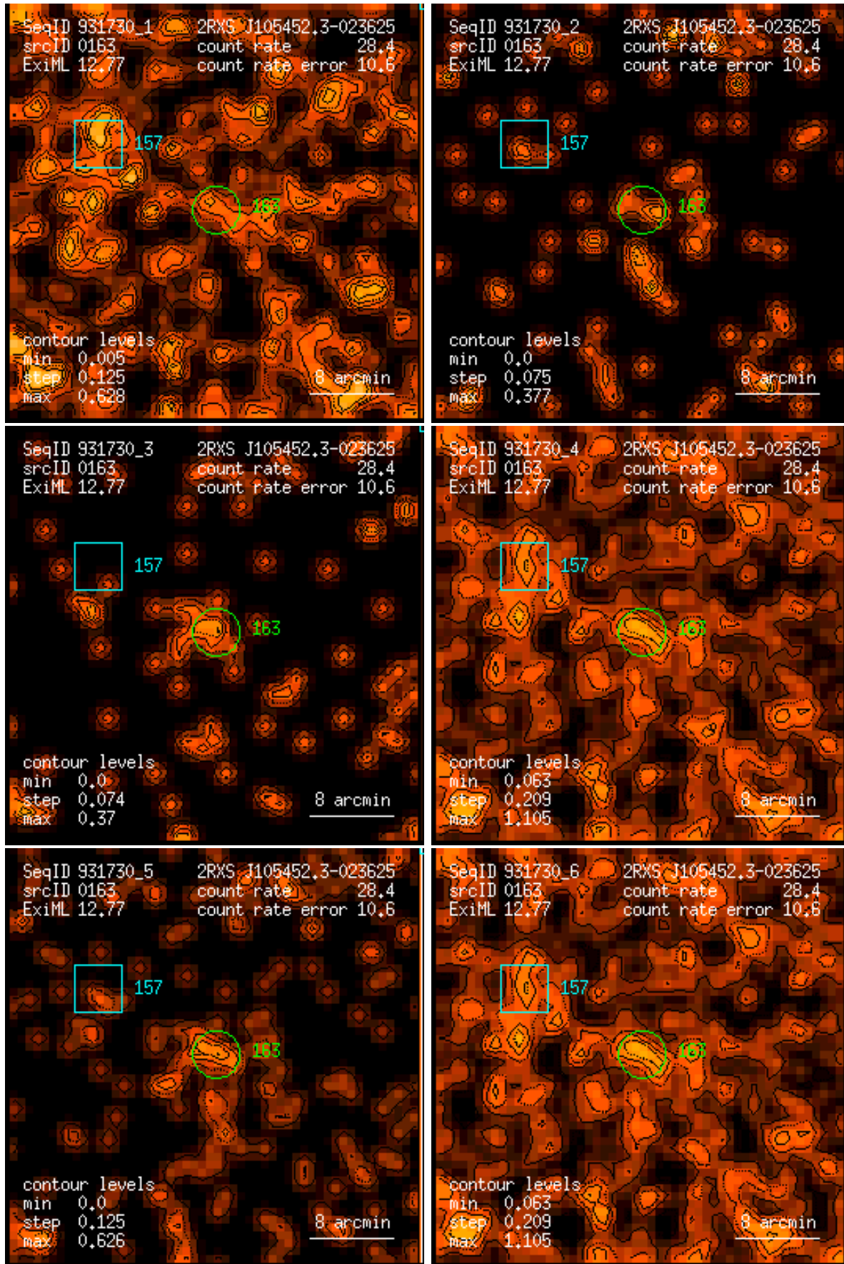
Figure 163: RASS 931730: detection 0163: band rate images, Gaussian filter: (1) PSPC channels 11 – 41, (2) 52 – 90, (3) 91 – 201, (4) 11 – 235, (5) 52 – 201, (6) 11 – 201. Broad band rates in counts/ks. Band rate contour levels in counts/ks/arcmin 2 .
