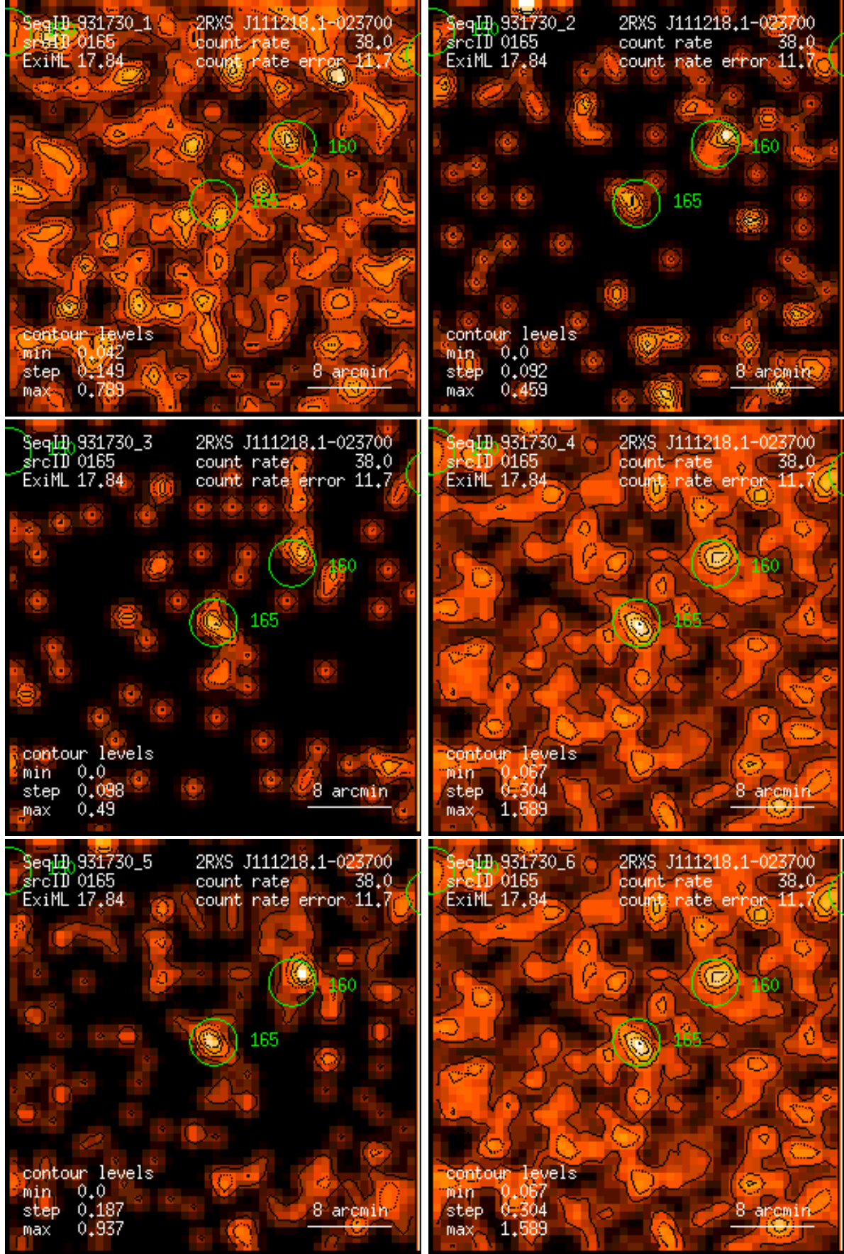
Figure 165: RASS 931730: detection 0165: band rate images, Gaussian filter: (1) PSPC channels 11 – 41, (2) 52 – 90, (3) 91 – 201, (4) 11 – 235, (5) 52 – 201, (6) 11 – 201. Broad band rates in counts/ks. Band rate contour levels in counts/ks/arcmin 2 .
