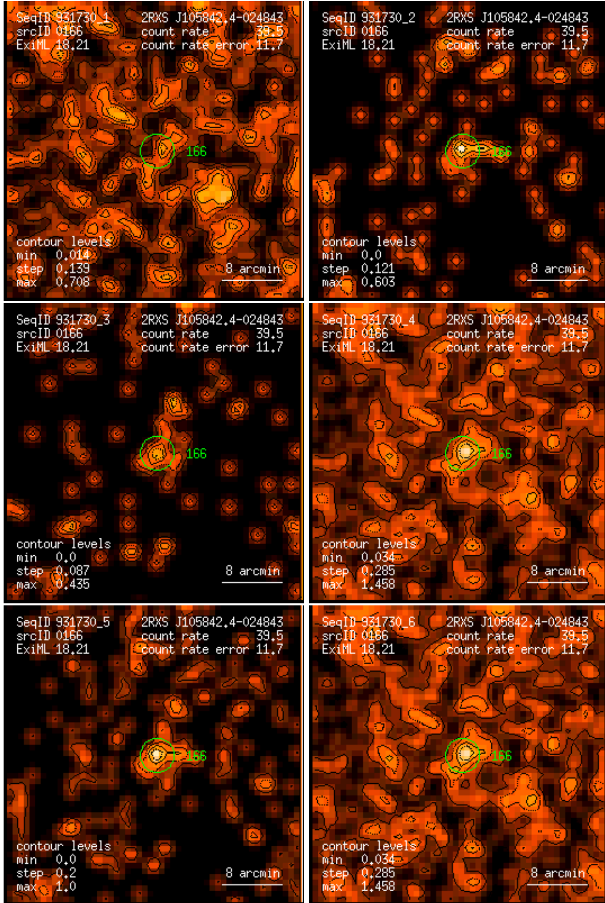
Figure 166: RASS 931730: detection 0166: band rate images, Gaussian filter: (1) PSPC channels 11 – 41, (2) 52 – 90, (3) 91 – 201, (4) 11 – 235, (5) 52 – 201, (6) 11 – 201. Broad band rates in counts/ks. Band rate contour levels in counts/ks/arcmin 2 .
