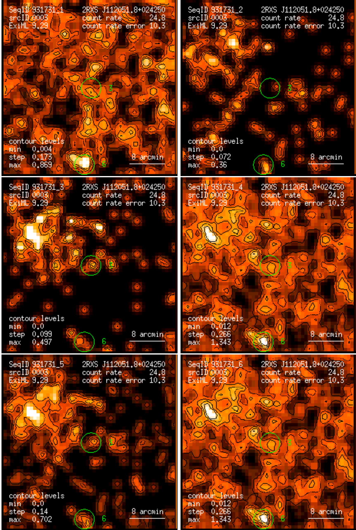
Figure 3: RASS 931731: detection 0003: band rate images, Gaussian filter: (1) PSPC channels 11 – 41, (2) 52 – 90, (3) 91 – 201, (4) 11 – 235, (5) 52 – 201, (6) 11 – 201. Broad band rates in counts/ks. Band rate contour levels in counts/ks/arcmin 2 .
