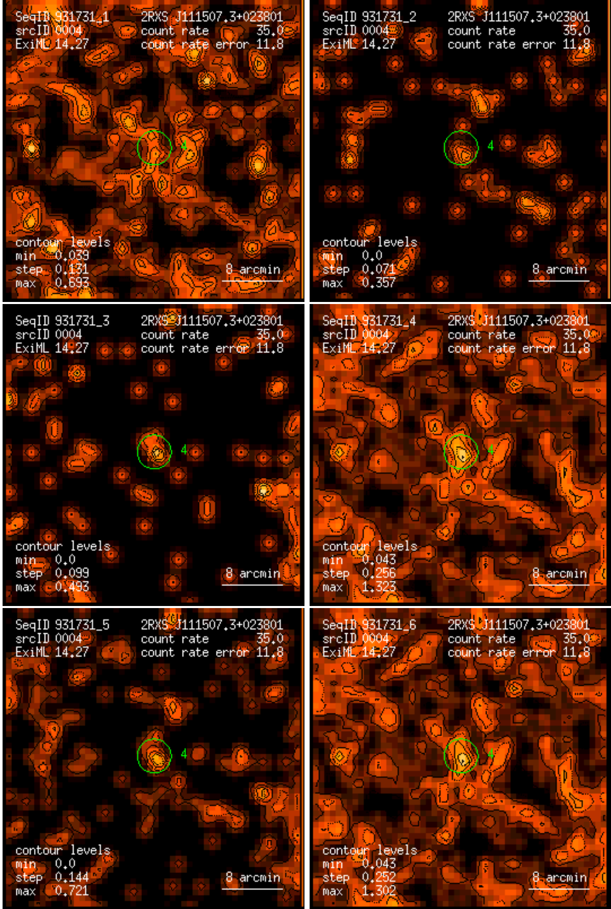
Figure 4: RASS 931731: detection 0004: band rate images, Gaussian filter: (1) PSPC channels 11 – 41, (2) 52 – 90, (3) 91 – 201, (4) 11 – 235, (5) 52 – 201, (6) 11 – 201. Broad band rates in counts/ks. Band rate contour levels in counts/ks/arcmin 2 .
