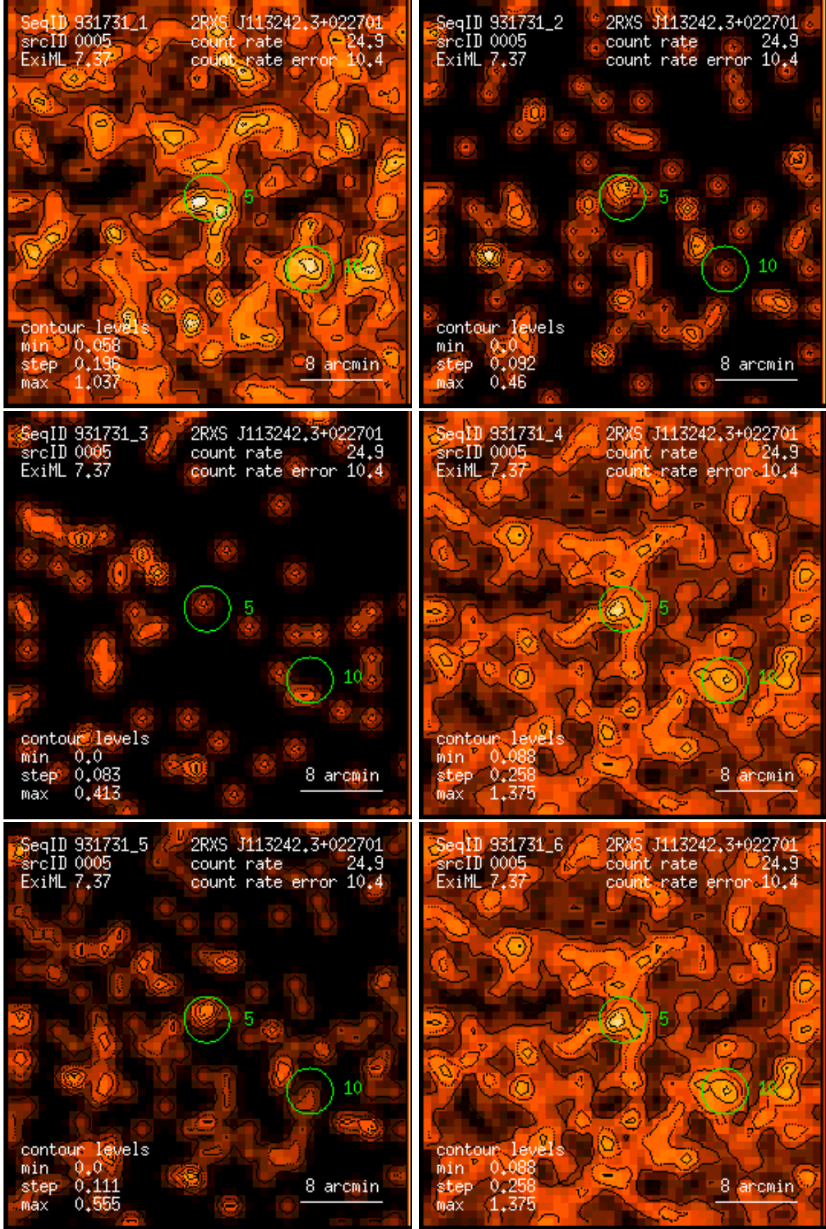
Figure 5: RASS 931731: detection 0005: band rate images, Gaussian filter: (1) PSPC channels 11 – 41, (2) 52 – 90, (3) 91 – 201, (4) 11 – 235, (5) 52 – 201, (6) 11 – 201. Broad band rates in counts/ks. Band rate contour levels in counts/ks/arcmin 2 .
