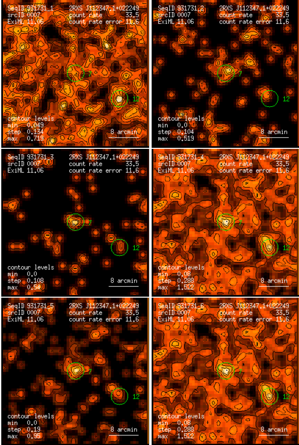
Figure 7: RASS 931731: detection 0007: band rate images, Gaussian filter: (1) PSPC channels 11 – 41, (2) 52 – 90, (3) 91 – 201, (4) 11 – 235, (5) 52 – 201, (6) 11 – 201. Broad band rates in counts/ks. Band rate contour levels in counts/ks/arcmin 2 .
