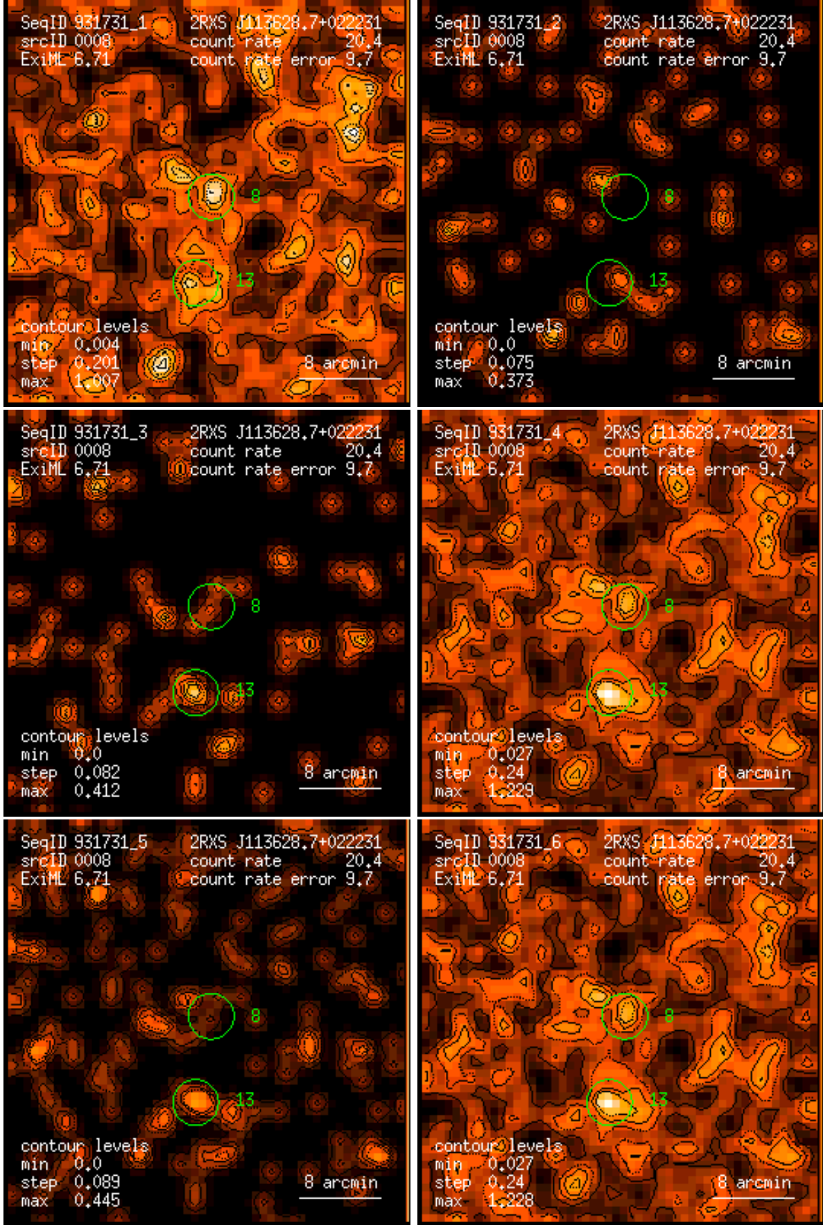
Figure 8: RASS 931731: detection 0008: band rate images, Gaussian filter: (1) PSPC channels 11 – 41, (2) 52 – 90, (3) 91 – 201, (4) 11 – 235, (5) 52 – 201, (6) 11 – 201. Broad band rates in counts/ks. Band rate contour levels in counts/ks/arcmin 2 .
