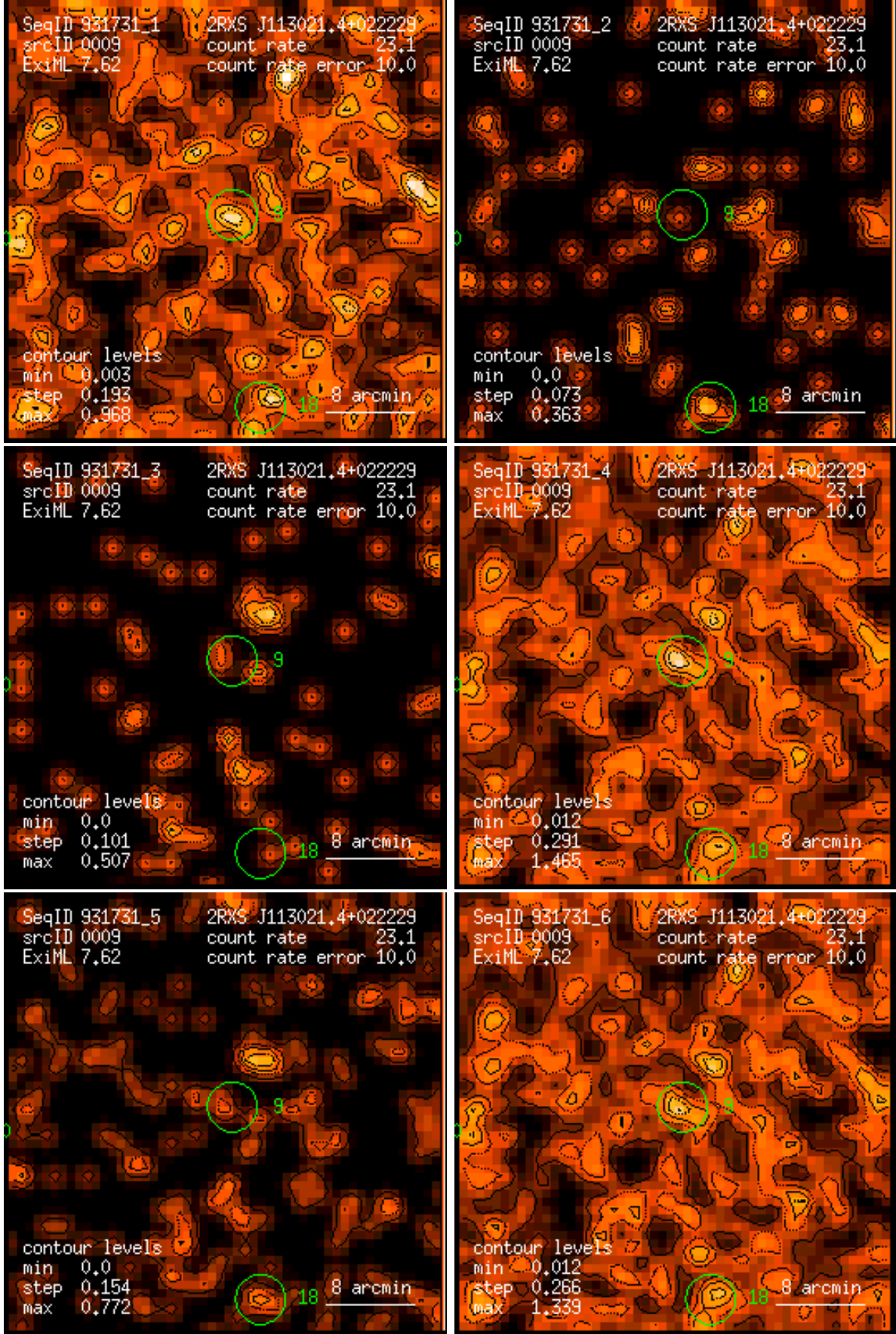
Figure 9: RASS 931731: detection 0009: band rate images, Gaussian filter: (1) PSPC channels 11 – 41, (2) 52 – 90, (3) 91 – 201, (4) 11 – 235, (5) 52 – 201, (6) 11 – 201. Broad band rates in counts/ks. Band rate contour levels in counts/ks/arcmin 2 .
