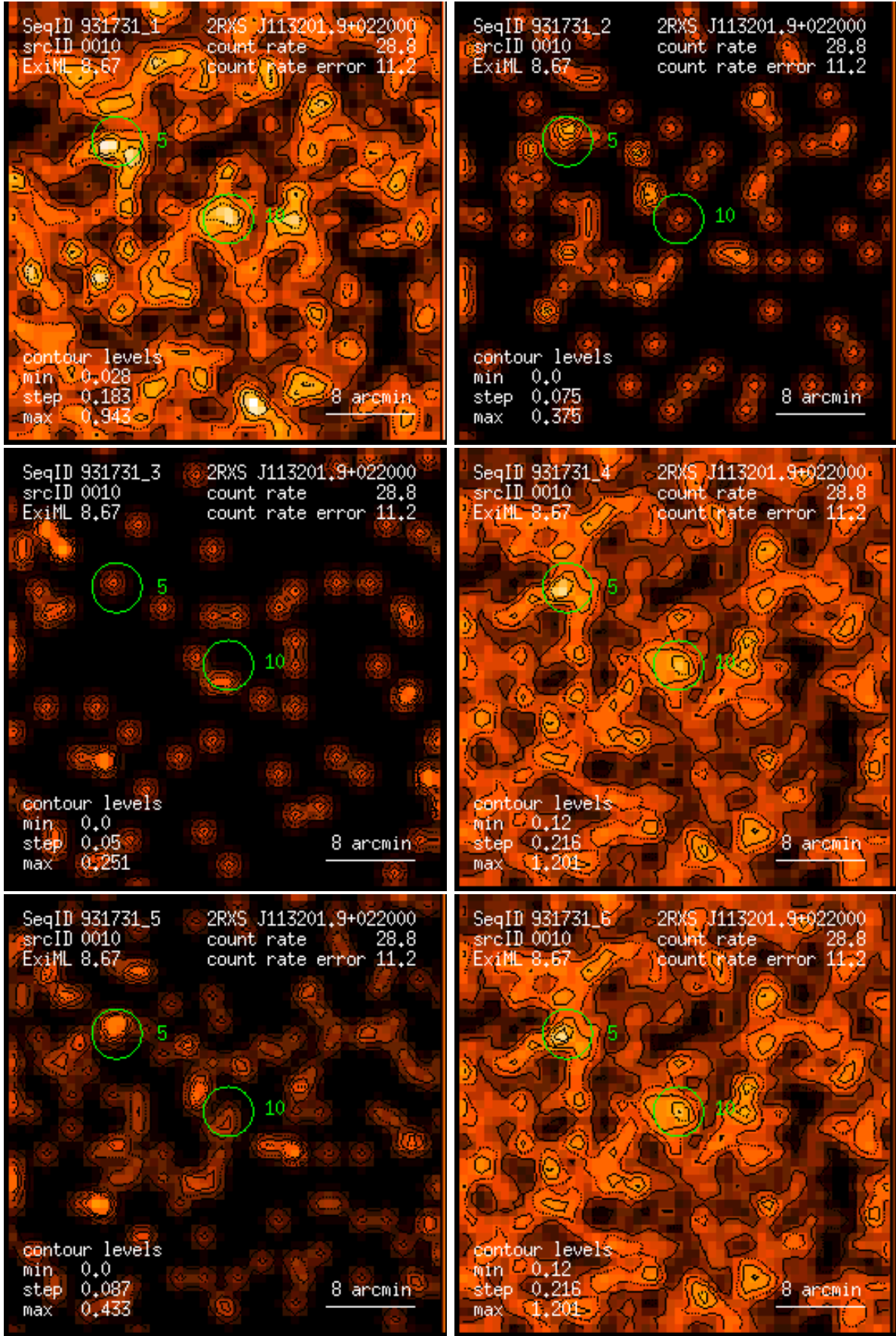
Figure 10: RASS 931731: detection 0010: band rate images, Gaussian filter: (1) PSPC channels 11 – 41, (2) 52 – 90, (3) 91 – 201, (4) 11 – 235, (5) 52 – 201, (6) 11 – 201. Broad band rates in counts/ks. Band rate contour levels in counts/ks/arcmin 2 .
