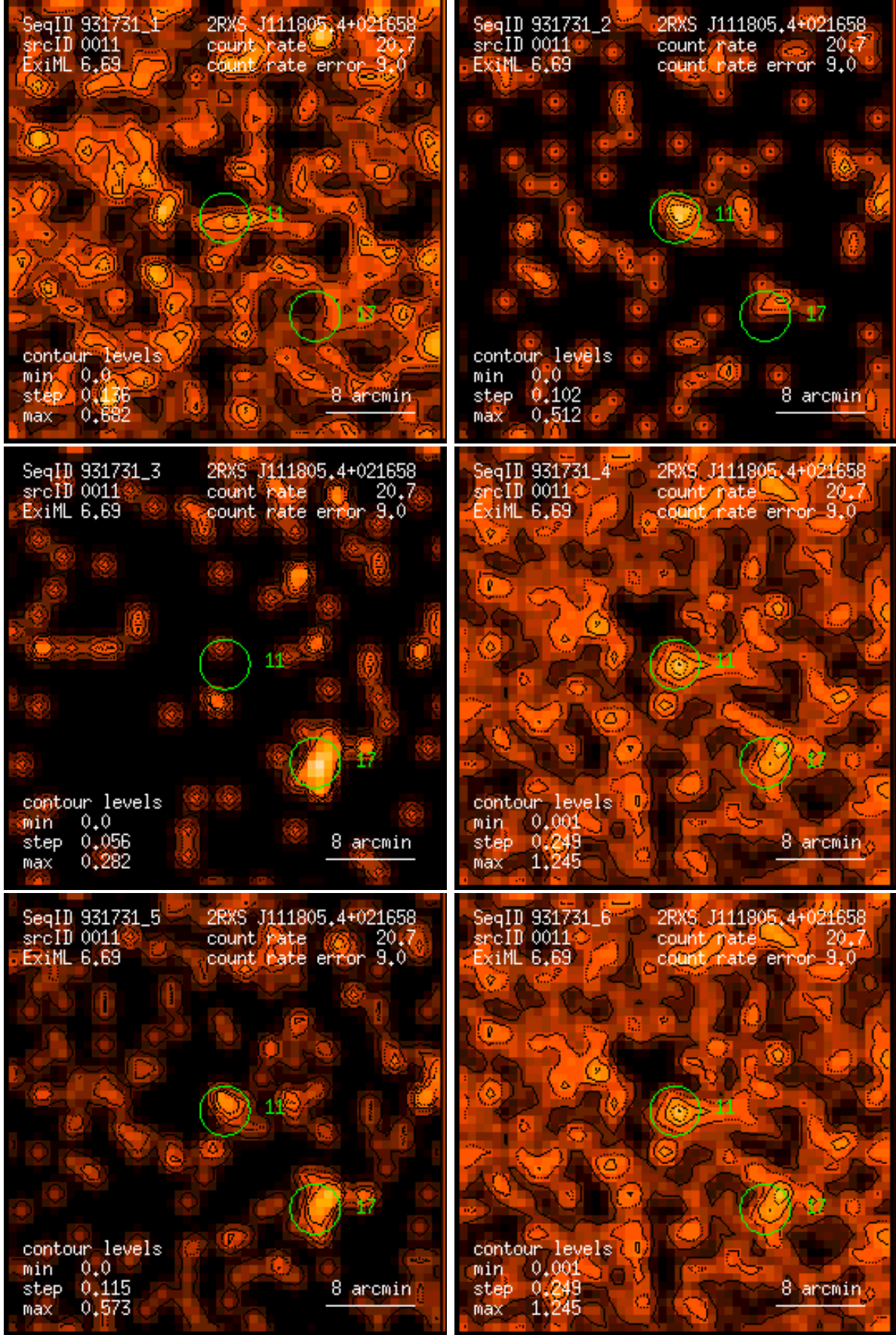
Figure 11: RASS 931731: detection 0011: band rate images, Gaussian filter: (1) PSPC channels 11 – 41, (2) 52 – 90, (3) 91 – 201, (4) 11 – 235, (5) 52 – 201, (6) 11 – 201. Broad band rates in counts/ks. Band rate contour levels in counts/ks/arcmin 2 .
