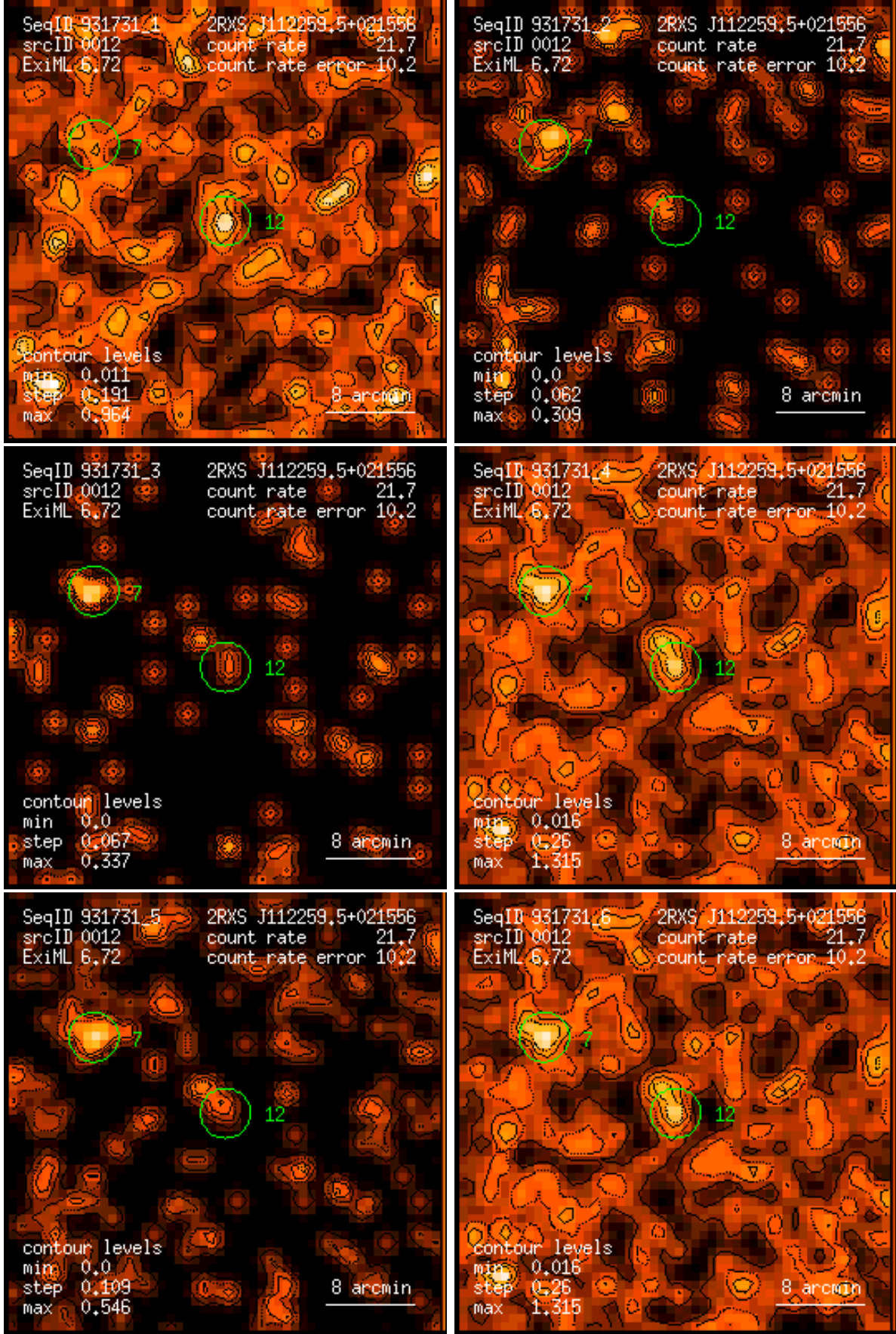
Figure 12: RASS 931731: detection 0012: band rate images, Gaussian filter: (1) PSPC channels 11 – 41, (2) 52 – 90, (3) 91 – 201, (4) 11 – 235, (5) 52 – 201, (6) 11 – 201. Broad band rates in counts/ks. Band rate contour levels in counts/ks/arcmin 2 .
