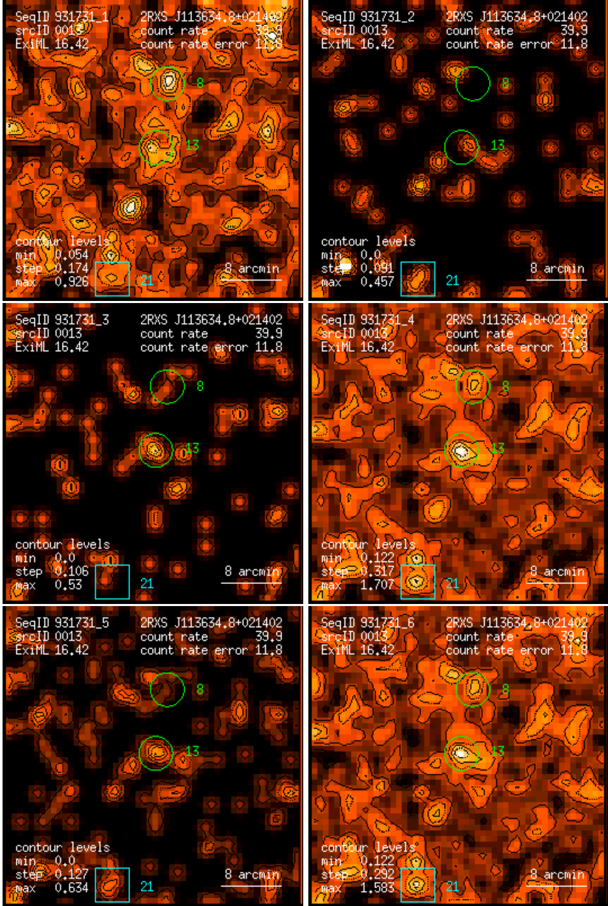
Figure 13: RASS 931731: detection 0013: band rate images, Gaussian filter: (1) PSPC channels 11 – 41, (2) 52 – 90, (3) 91 – 201, (4) 11 – 235, (5) 52 – 201, (6) 11 – 201. Broad band rates in counts/ks. Band rate contour levels in counts/ks/arcmin 2 .
