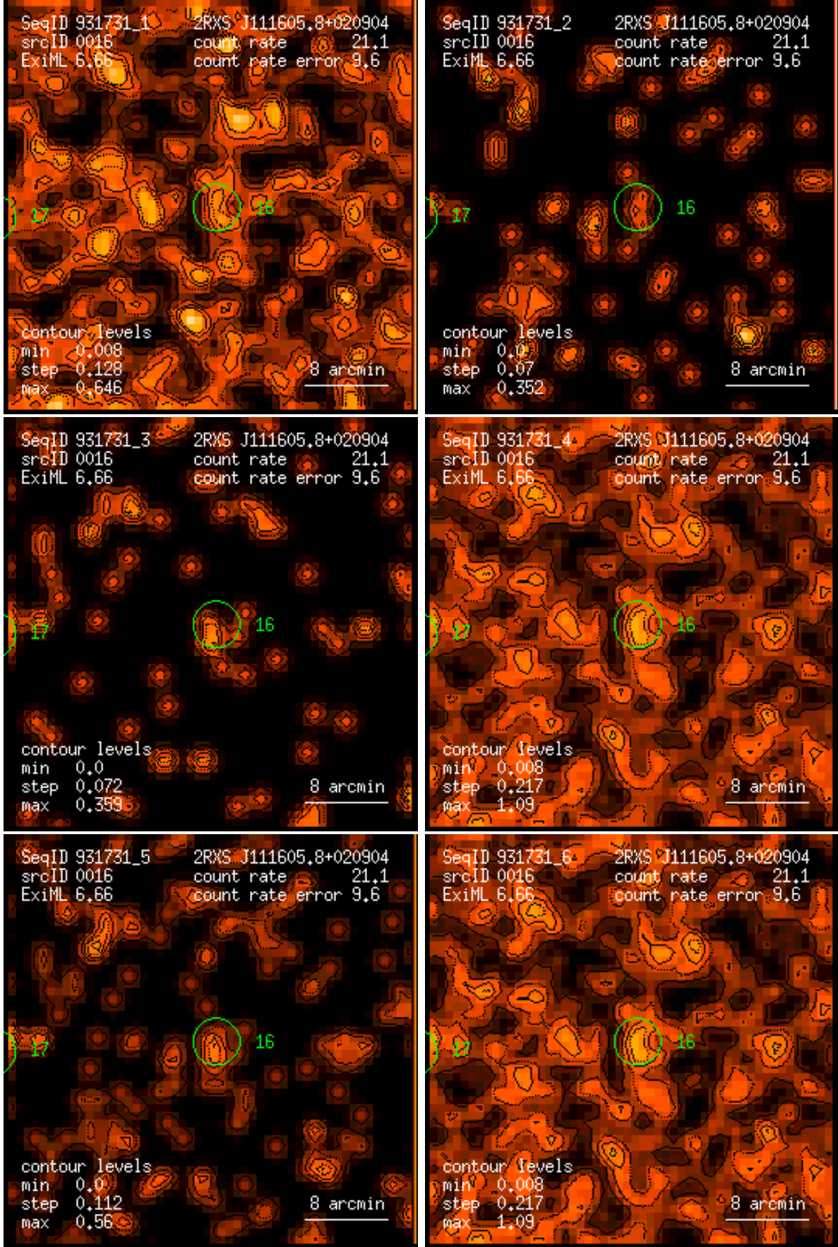
Figure 16: RASS 931731: detection 0016: band rate images, Gaussian filter: (1) PSPC channels 11 – 41, (2) 52 – 90, (3) 91 – 201, (4) 11 – 235, (5) 52 – 201, (6) 11 – 201. Broad band rates in counts/ks. Band rate contour levels in counts/ks/arcmin 2 .
