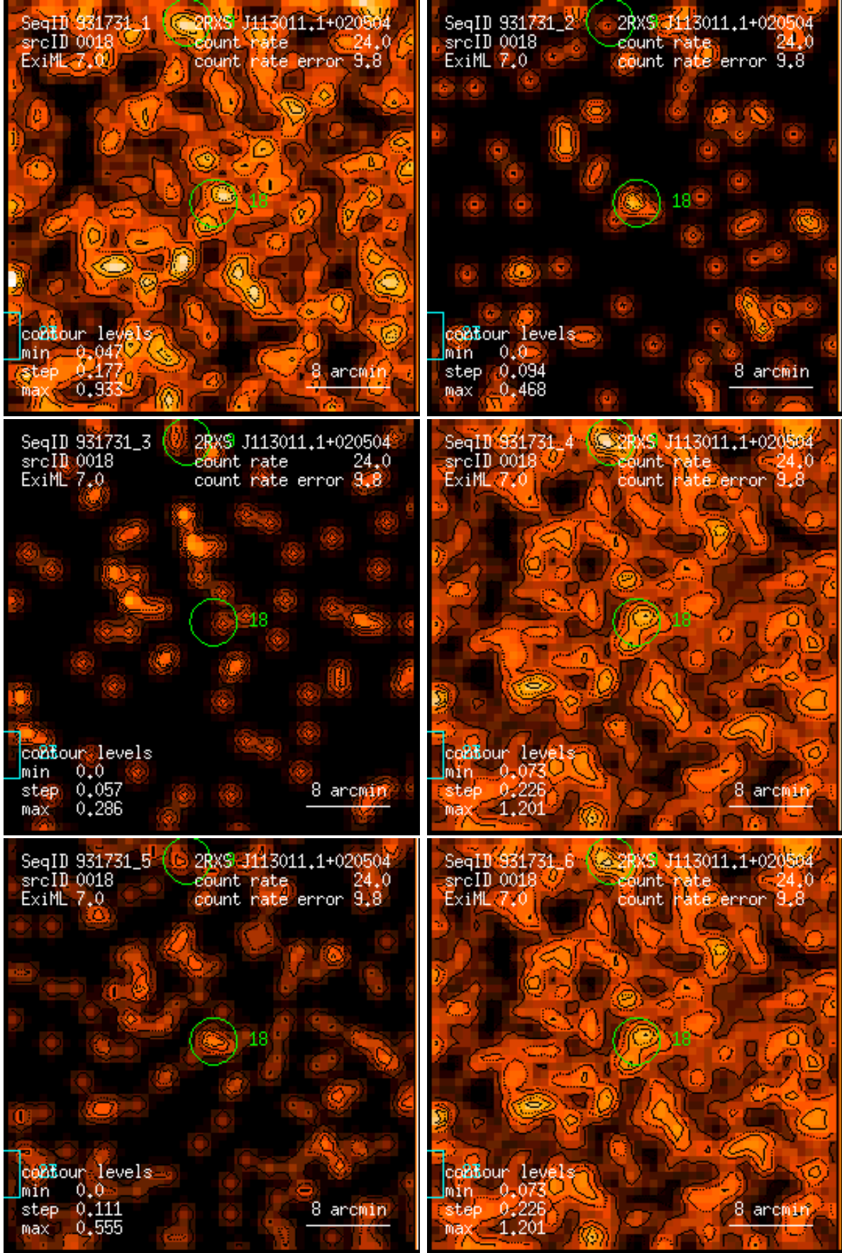
Figure 18: RASS 931731: detection 0018: band rate images, Gaussian filter: (1) PSPC channels 11 – 41, (2) 52 – 90, (3) 91 – 201, (4) 11 – 235, (5) 52 – 201, (6) 11 – 201. Broad band rates in counts/ks. Band rate contour levels in counts/ks/arcmin 2 .
