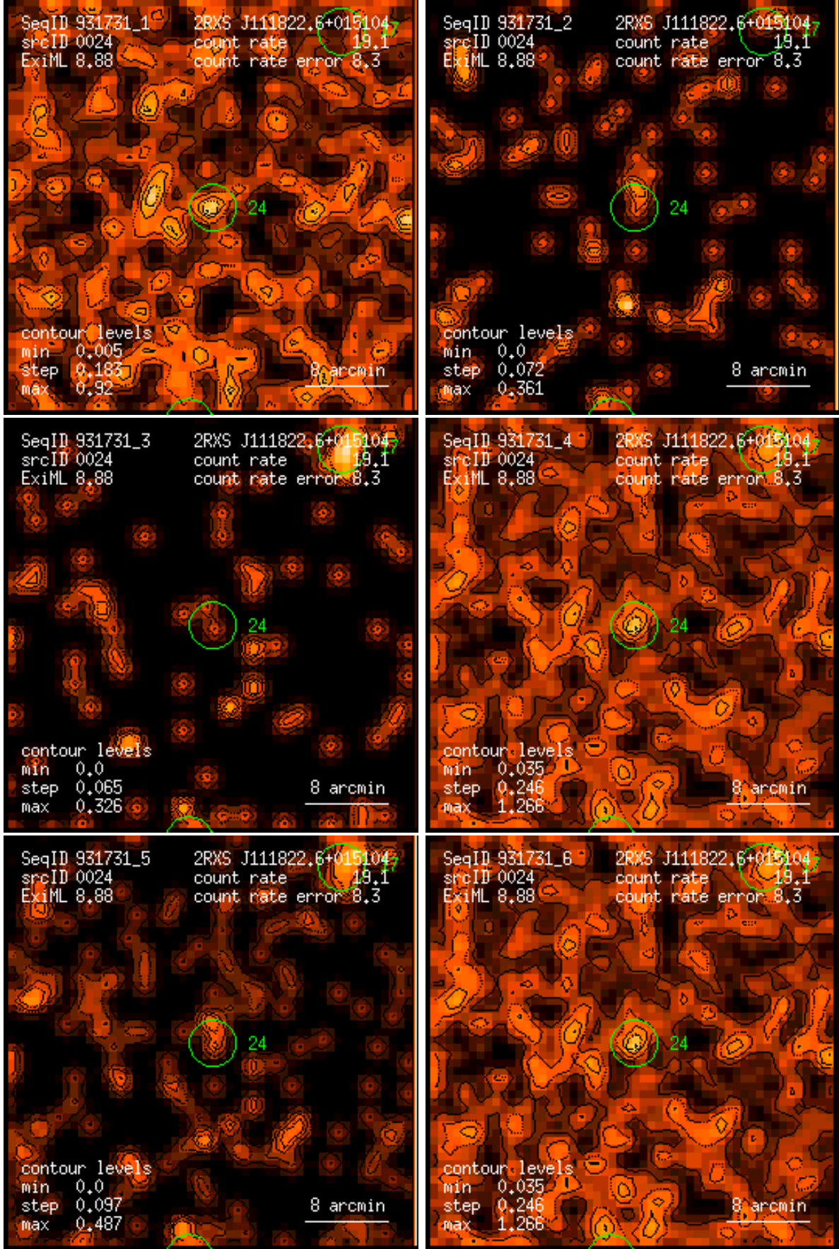
Figure 24: RASS 931731: detection 0024: band rate images, Gaussian filter: (1) PSPC channels 11 – 41, (2) 52 – 90, (3) 91 – 201, (4) 11 – 235, (5) 52 – 201, (6) 11 – 201. Broad band rates in counts/ks. Band rate contour levels in counts/ks/arcmin 2 .
