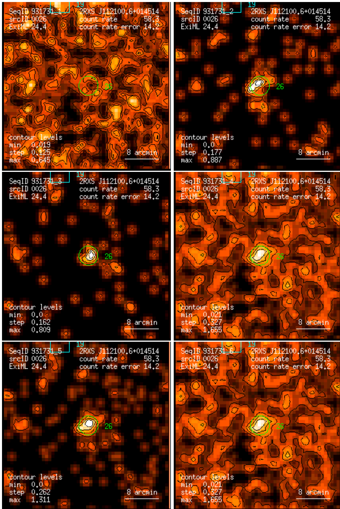
Figure 26: RASS 931731: detection 0026: band rate images, Gaussian filter: (1) PSPC channels 11 – 41, (2) 52 – 90, (3) 91 – 201, (4) 11 – 235, (5) 52 – 201, (6) 11 – 201. Broad band rates in counts/ks. Band rate contour levels in counts/ks/arcmin 2 .
