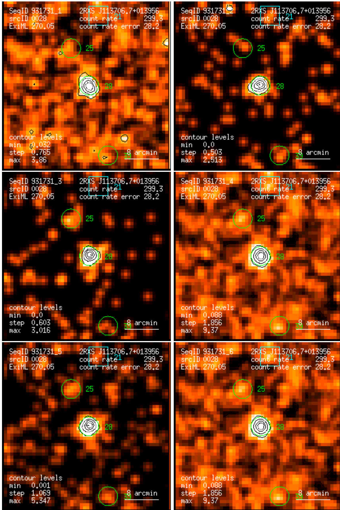
Figure 28: RASS 931731: detection 0028: band rate images, Gaussian filter: (1) PSPC channels 11 – 41, (2) 52 – 90, (3) 91 – 201, (4) 11 – 235, (5) 52 – 201, (6) 11 – 201. Broad band rates in counts/ks. Band rate contour levels in counts/ks/arcmin 2 .
