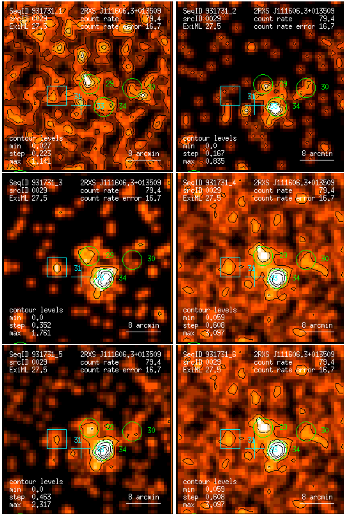
Figure 29: RASS 931731: detection 0029: band rate images, Gaussian filter: (1) PSPC channels 11 – 41, (2) 52 – 90, (3) 91 – 201, (4) 11 – 235, (5) 52 – 201, (6) 11 – 201. Broad band rates in counts/ks. Band rate contour levels in counts/ks/arcmin 2 .
