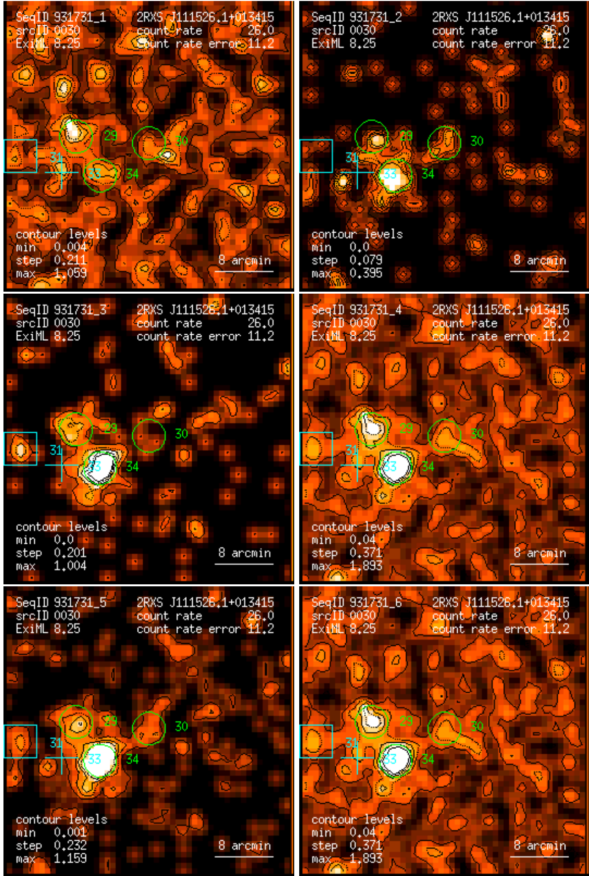
Figure 30: RASS 931731: detection 0030: band rate images, Gaussian filter: (1) PSPC channels 11 – 41, (2) 52 – 90, (3) 91 – 201, (4) 11 – 235, (5) 52 – 201, (6) 11 – 201. Broad band rates in counts/ks. Band rate contour levels in counts/ks/arcmin 2 .
