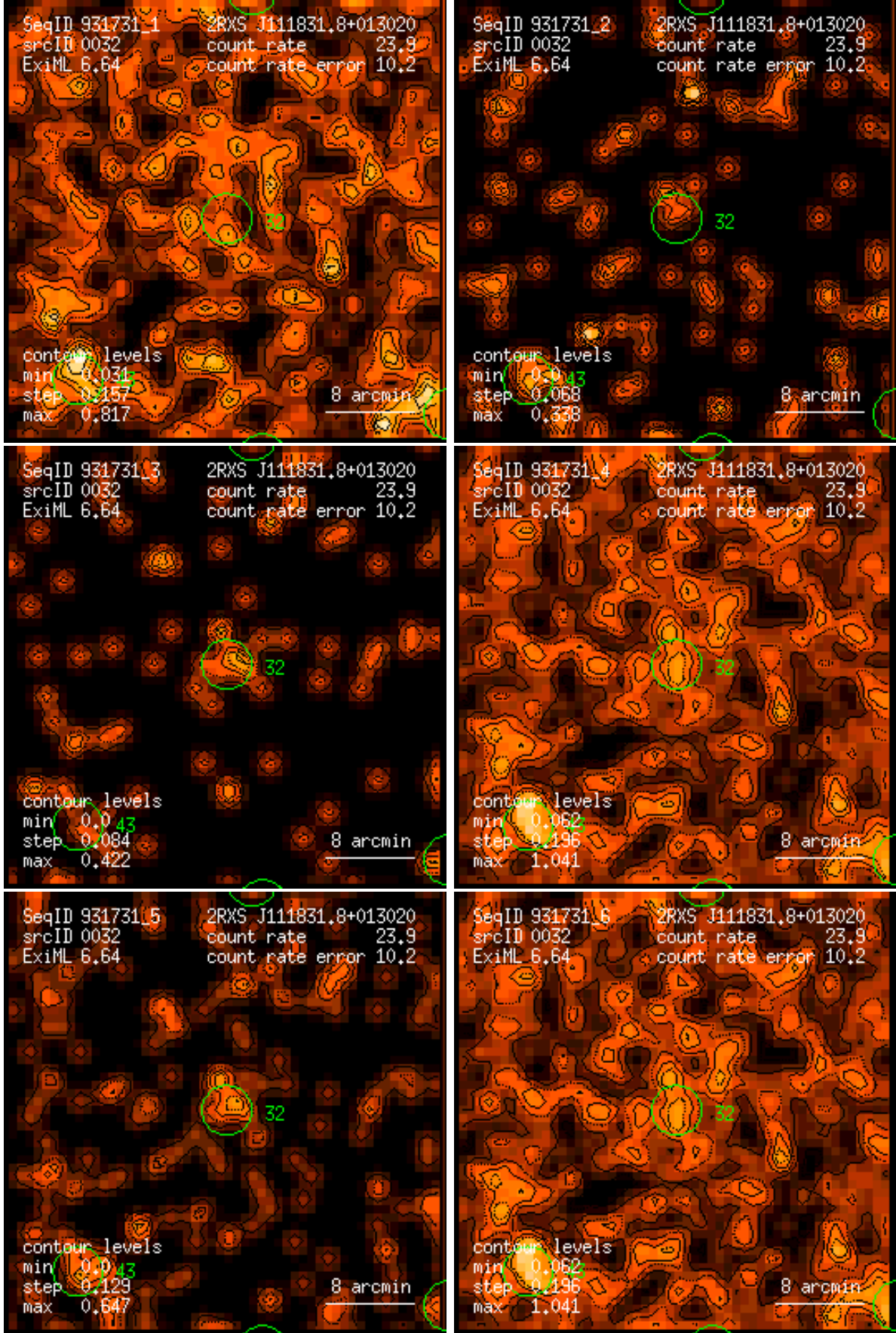
Figure 32: RASS 931731: detection 0032: band rate images, Gaussian filter: (1) PSPC channels 11 – 41, (2) 52 – 90, (3) 91 – 201, (4) 11 – 235, (5) 52 – 201, (6) 11 – 201. Broad band rates in counts/ks. Band rate contour levels in counts/ks/arcmin 2 .
