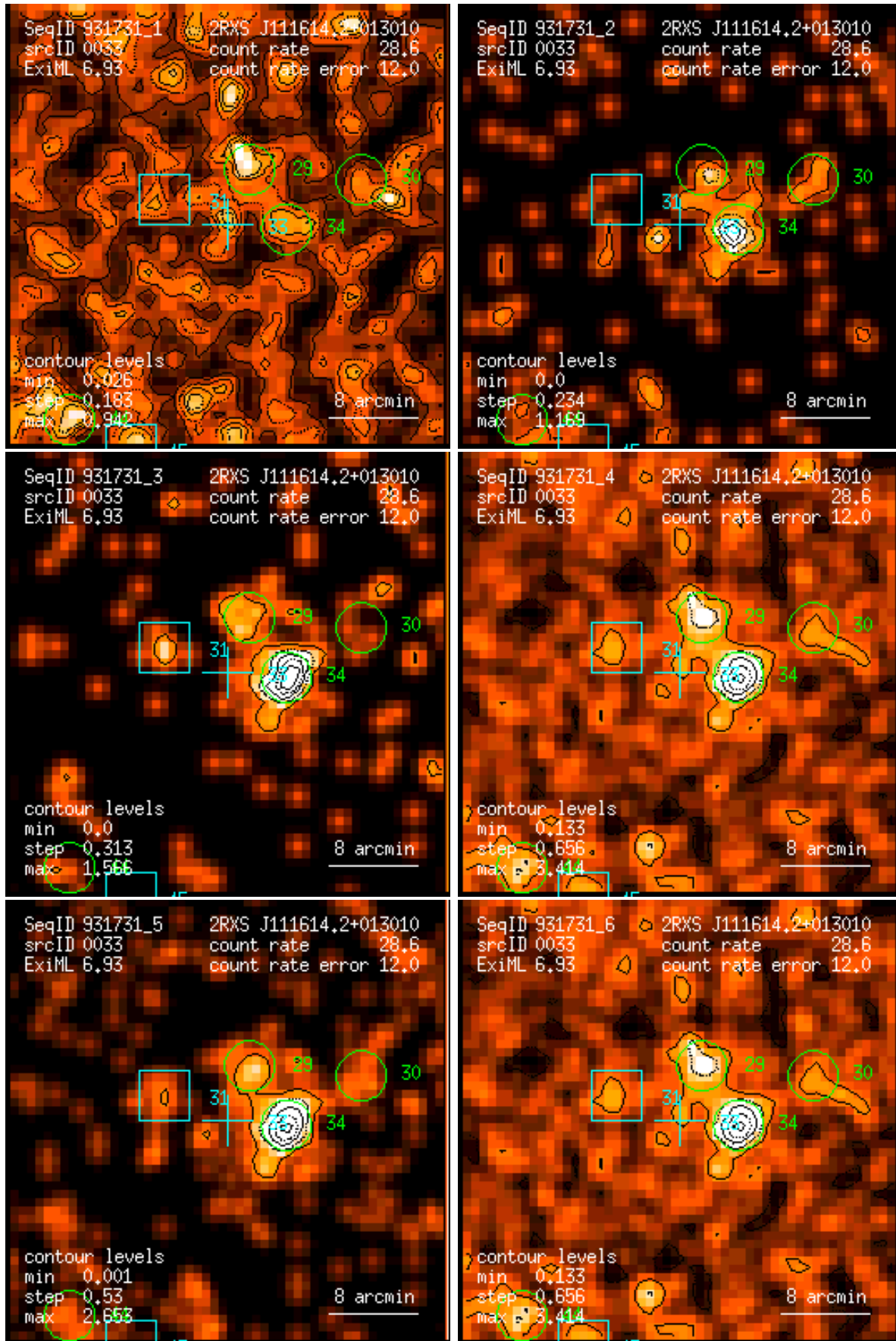
Figure 33: RASS 931731: detection 0033: band rate images, Gaussian filter: (1) PSPC channels 11 – 41, (2) 52 – 90, (3) 91 – 201, (4) 11 – 235, (5) 52 – 201, (6) 11 – 201. Broad band rates in counts/ks. Band rate contour levels in counts/ks/arcmin 2 .
