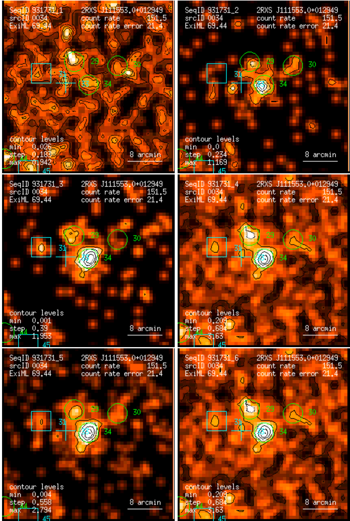
Figure 34: RASS 931731: detection 0034: band rate images, Gaussian filter: (1) PSPC channels 11 – 41, (2) 52 – 90, (3) 91 – 201, (4) 11 – 235, (5) 52 – 201, (6) 11 – 201. Broad band rates in counts/ks. Band rate contour levels in counts/ks/arcmin 2 .
