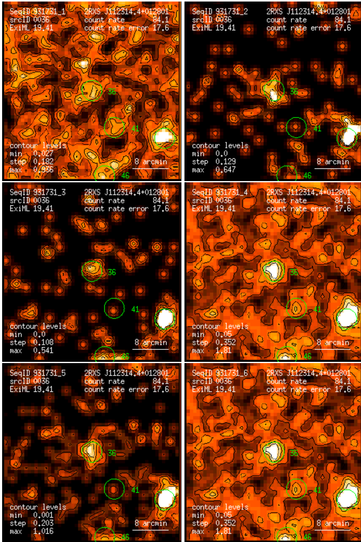
Figure 36: RASS 931731: detection 0036: band rate images, Gaussian filter: (1) PSPC channels 11 – 41, (2) 52 – 90, (3) 91 – 201, (4) 11 – 235, (5) 52 – 201, (6) 11 – 201. Broad band rates in counts/ks. Band rate contour levels in counts/ks/arcmin 2 .
