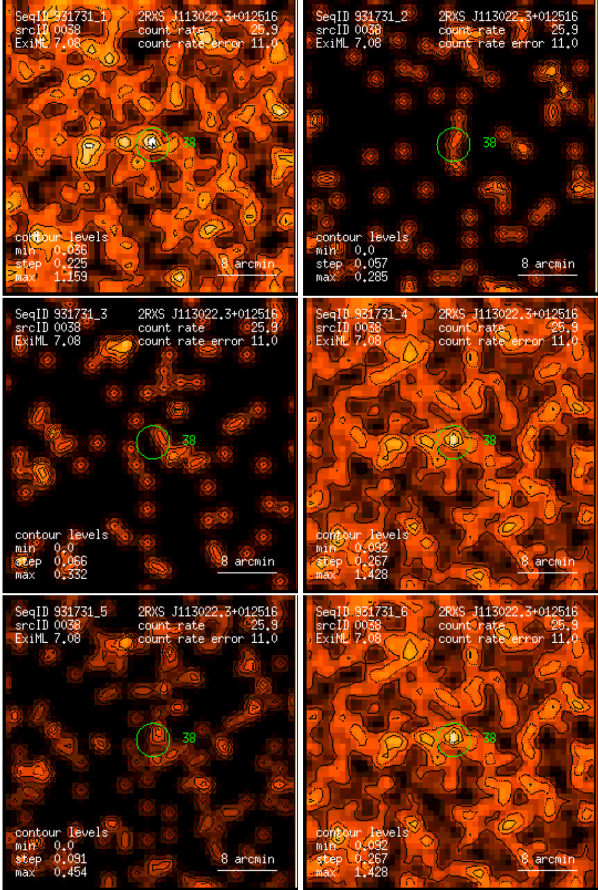
Figure 38: RASS 931731: detection 0038: band rate images, Gaussian filter: (1) PSPC channels 11 – 41, (2) 52 – 90, (3) 91 – 201, (4) 11 – 235, (5) 52 – 201, (6) 11 – 201. Broad band rates in counts/ks. Band rate contour levels in counts/ks/arcmin 2 .
