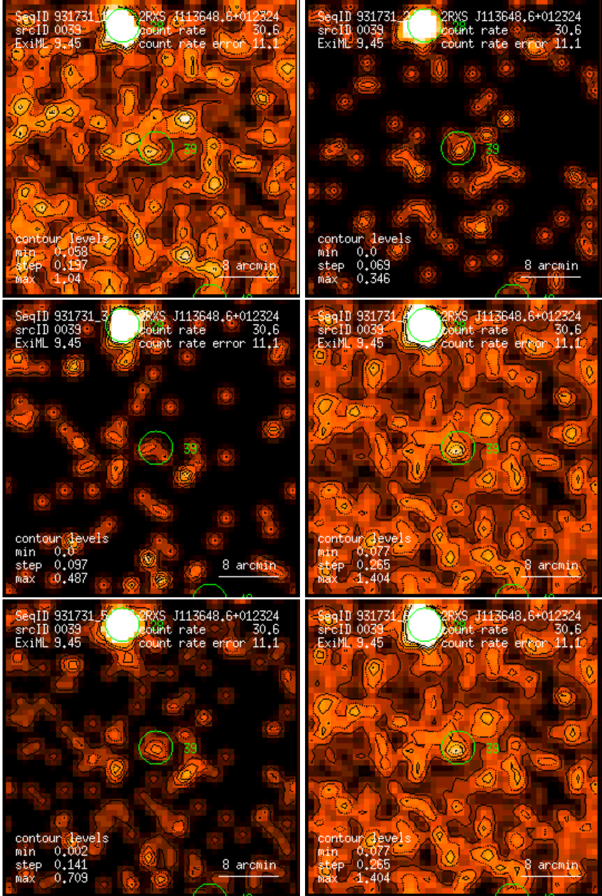
Figure 39: RASS 931731: detection 0039: band rate images, Gaussian filter: (1) PSPC channels 11 – 41, (2) 52 – 90, (3) 91 – 201, (4) 11 – 235, (5) 52 – 201, (6) 11 – 201. Broad band rates in counts/ks. Band rate contour levels in counts/ks/arcmin 2 .
