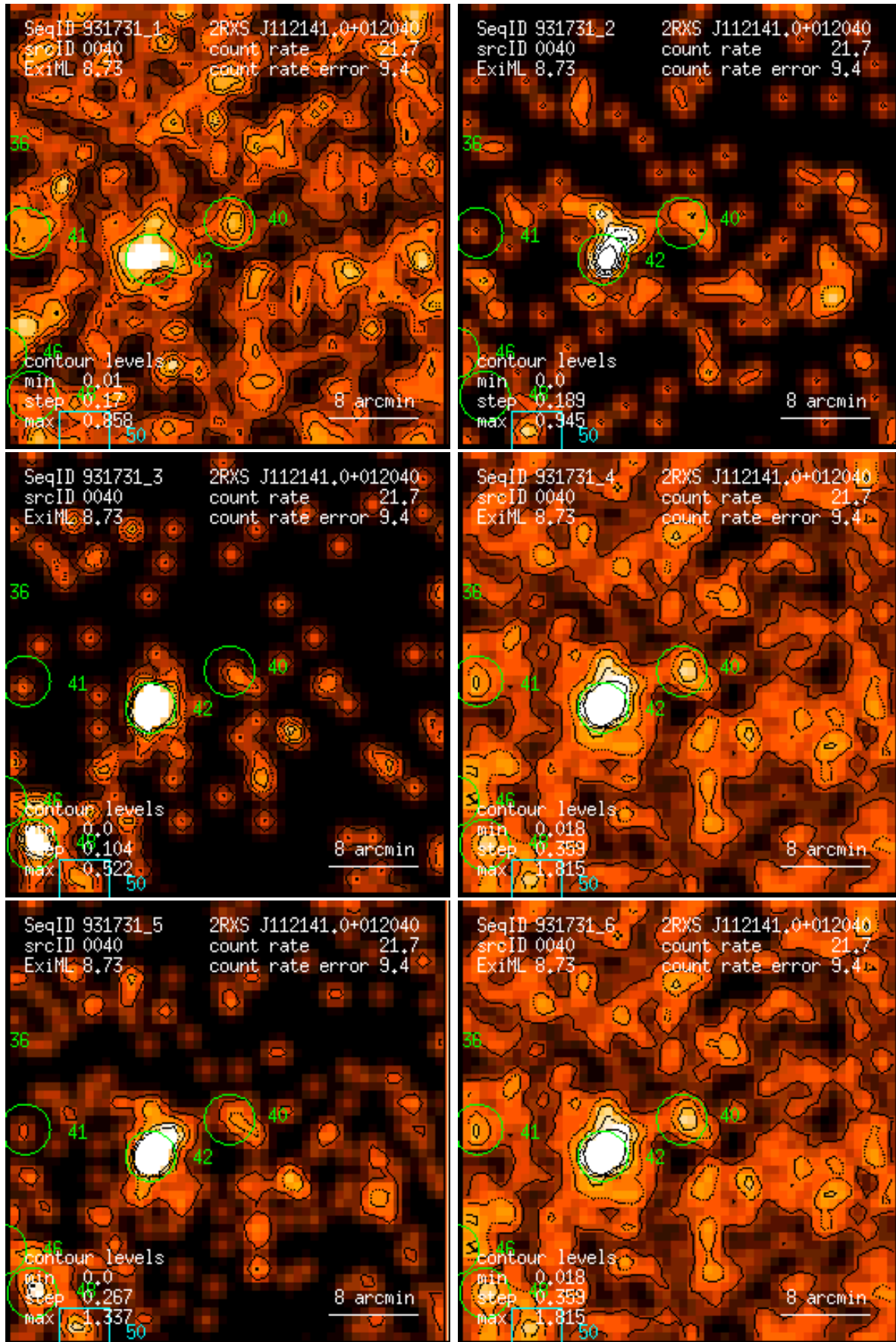
Figure 40: RASS 931731: detection 0040: band rate images, Gaussian filter: (1) PSPC channels 11 – 41, (2) 52 – 90, (3) 91 – 201, (4) 11 – 235, (5) 52 – 201, (6) 11 – 201. Broad band rates in counts/ks. Band rate contour levels in counts/ks/arcmin 2 .
