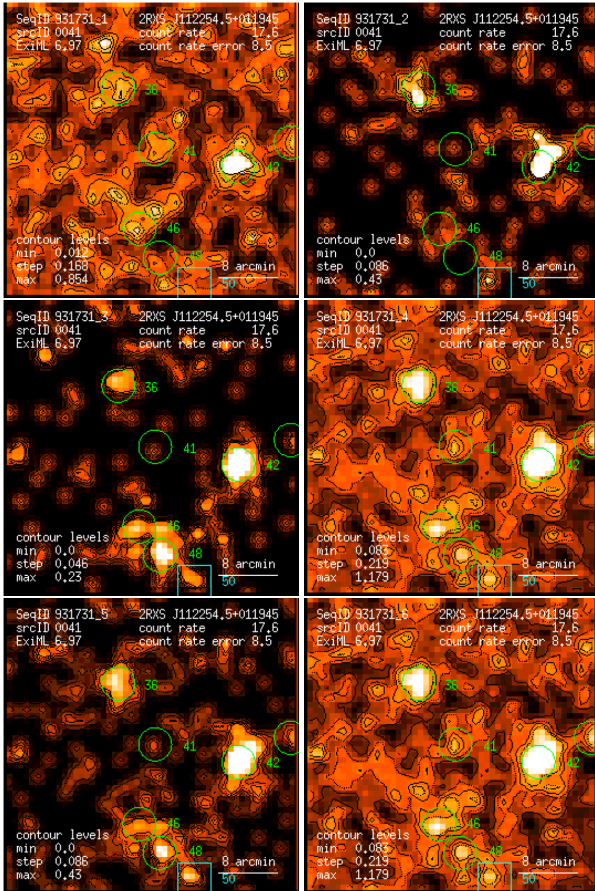
Figure 41: RASS 931731: detection 0041: band rate images, Gaussian filter: (1) PSPC channels 11 – 41, (2) 52 – 90, (3) 91 – 201, (4) 11 – 235, (5) 52 – 201, (6) 11 – 201. Broad band rates in counts/ks. Band rate contour levels in counts/ks/arcmin 2 .
