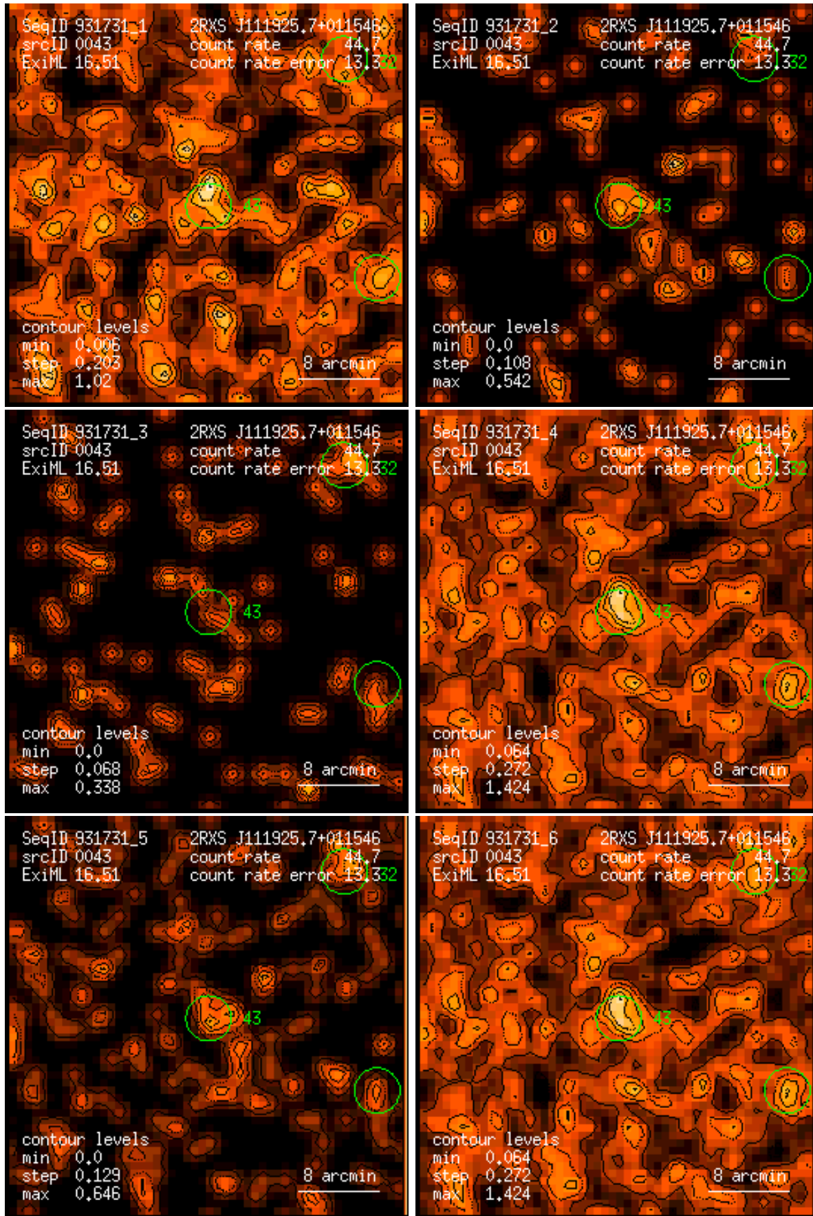
Figure 43: RASS 931731: detection 0043: band rate images, Gaussian filter: (1) PSPC channels 11 – 41, (2) 52 – 90, (3) 91 – 201, (4) 11 – 235, (5) 52 – 201, (6) 11 – 201. Broad band rates in counts/ks. Band rate contour levels in counts/ks/arcmin 2 .
