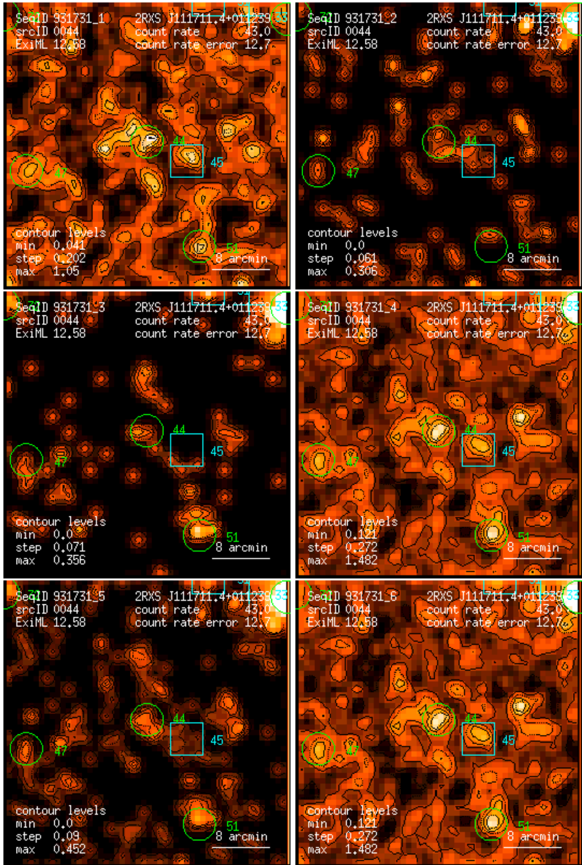
Figure 44: RASS 931731: detection 0044: band rate images, Gaussian filter: (1) PSPC channels 11 – 41, (2) 52 – 90, (3) 91 – 201, (4) 11 – 235, (5) 52 – 201, (6) 11 – 201. Broad band rates in counts/ks. Band rate contour levels in counts/ks/arcmin 2 .
