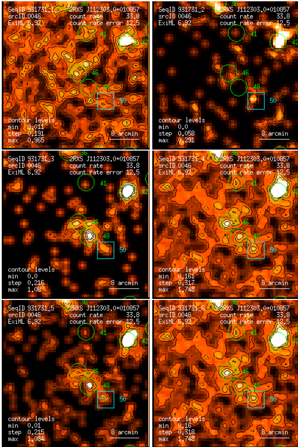
Figure 46: RASS 931731: detection 0046: band rate images, Gaussian filter: (1) PSPC channels 11 – 41, (2) 52 – 90, (3) 91 – 201, (4) 11 – 235, (5) 52 – 201, (6) 11 – 201. Broad band rates in counts/ks. Band rate contour levels in counts/ks/arcmin 2 .
