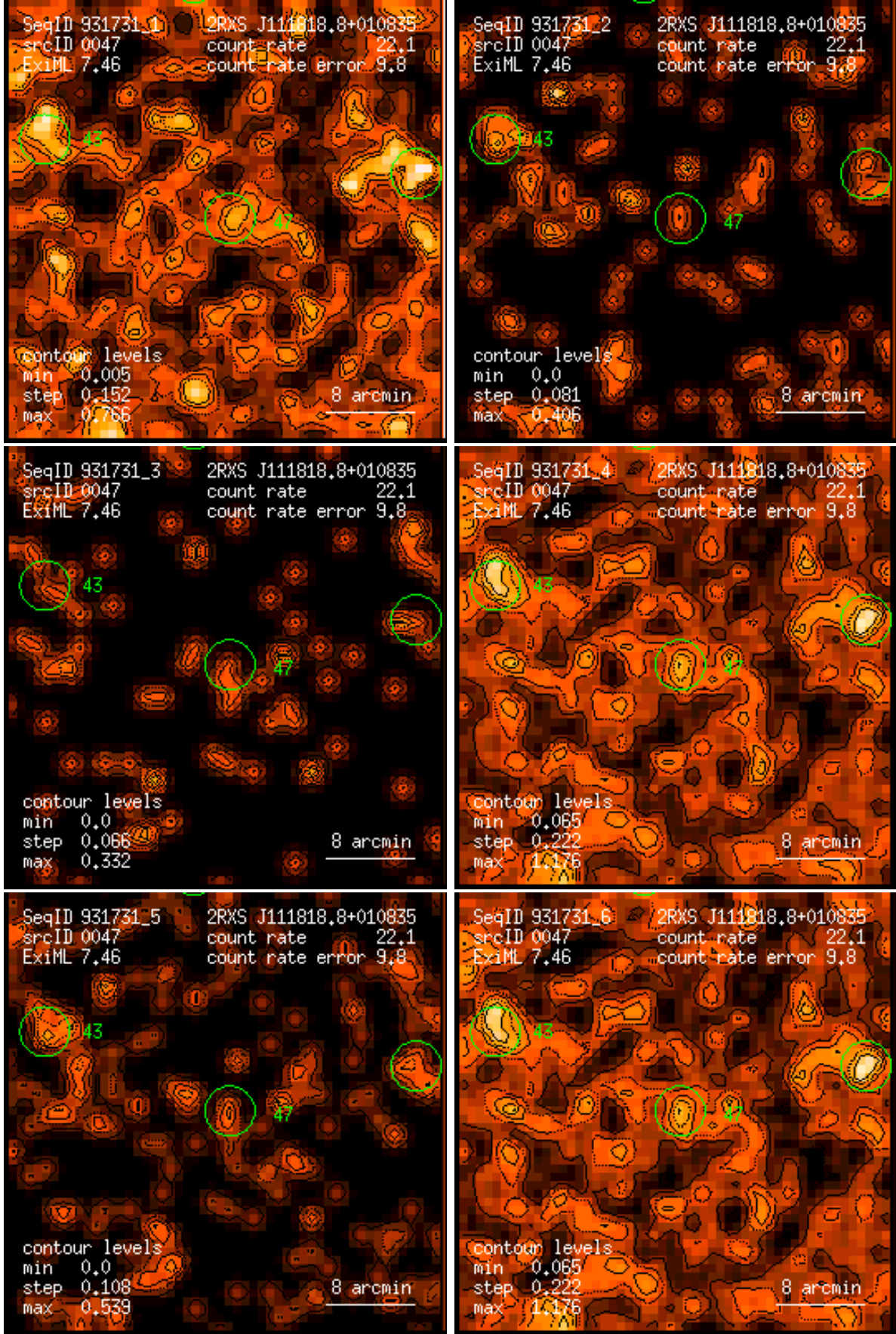
Figure 47: RASS 931731: detection 0047: band rate images, Gaussian filter: (1) PSPC channels 11 – 41, (2) 52 – 90, (3) 91 – 201, (4) 11 – 235, (5) 52 – 201, (6) 11 – 201. Broad band rates in counts/ks. Band rate contour levels in counts/ks/arcmin 2 .
