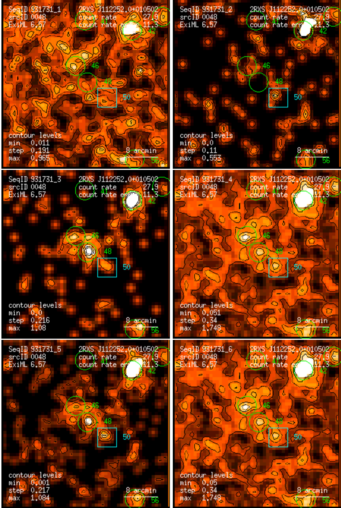
Figure 48: RASS 931731: detection 0048: band rate images, Gaussian filter: (1) PSPC channels 11 – 41, (2) 52 – 90, (3) 91 – 201, (4) 11 – 235, (5) 52 – 201, (6) 11 – 201. Broad band rates in counts/ks. Band rate contour levels in counts/ks/arcmin 2 .
