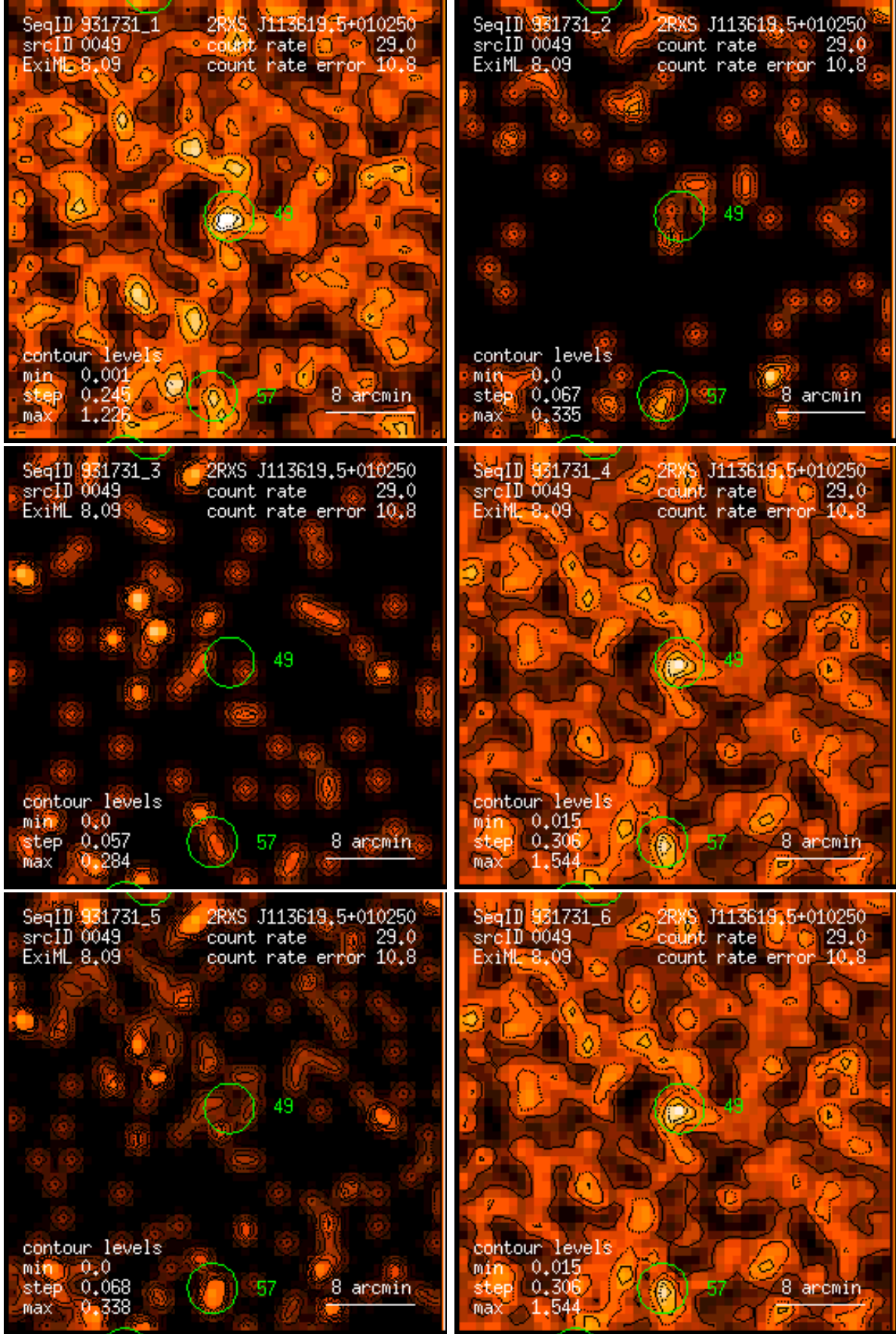
Figure 49: RASS 931731: detection 0049: band rate images, Gaussian filter: (1) PSPC channels 11 – 41, (2) 52 – 90, (3) 91 – 201, (4) 11 – 235, (5) 52 – 201, (6) 11 – 201. Broad band rates in counts/ks. Band rate contour levels in counts/ks/arcmin 2 .
