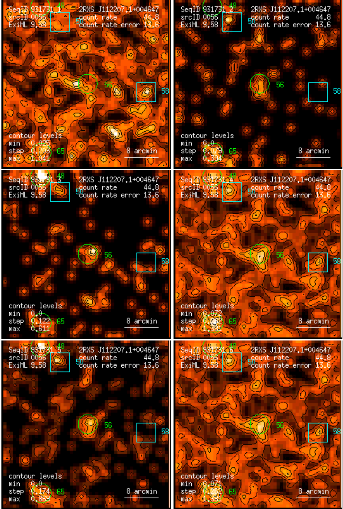
Figure 56: RASS 931731: detection 0056: band rate images, Gaussian filter: (1) PSPC channels 11 – 41, (2) 52 – 90, (3) 91 – 201, (4) 11 – 235, (5) 52 – 201, (6) 11 – 201. Broad band rates in counts/ks. Band rate contour levels in counts/ks/arcmin 2 .
