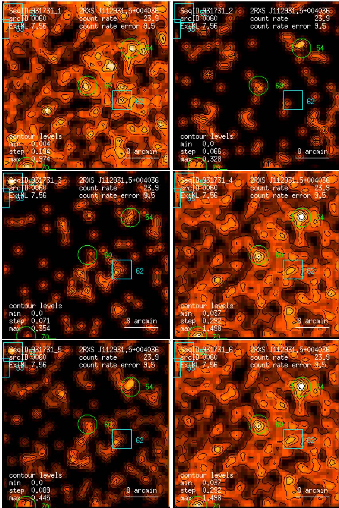
Figure 60: RASS 931731: detection 0060: band rate images, Gaussian filter: (1) PSPC channels 11 – 41, (2) 52 – 90, (3) 91 – 201, (4) 11 – 235, (5) 52 – 201, (6) 11 – 201. Broad band rates in counts/ks. Band rate contour levels in counts/ks/arcmin 2 .
