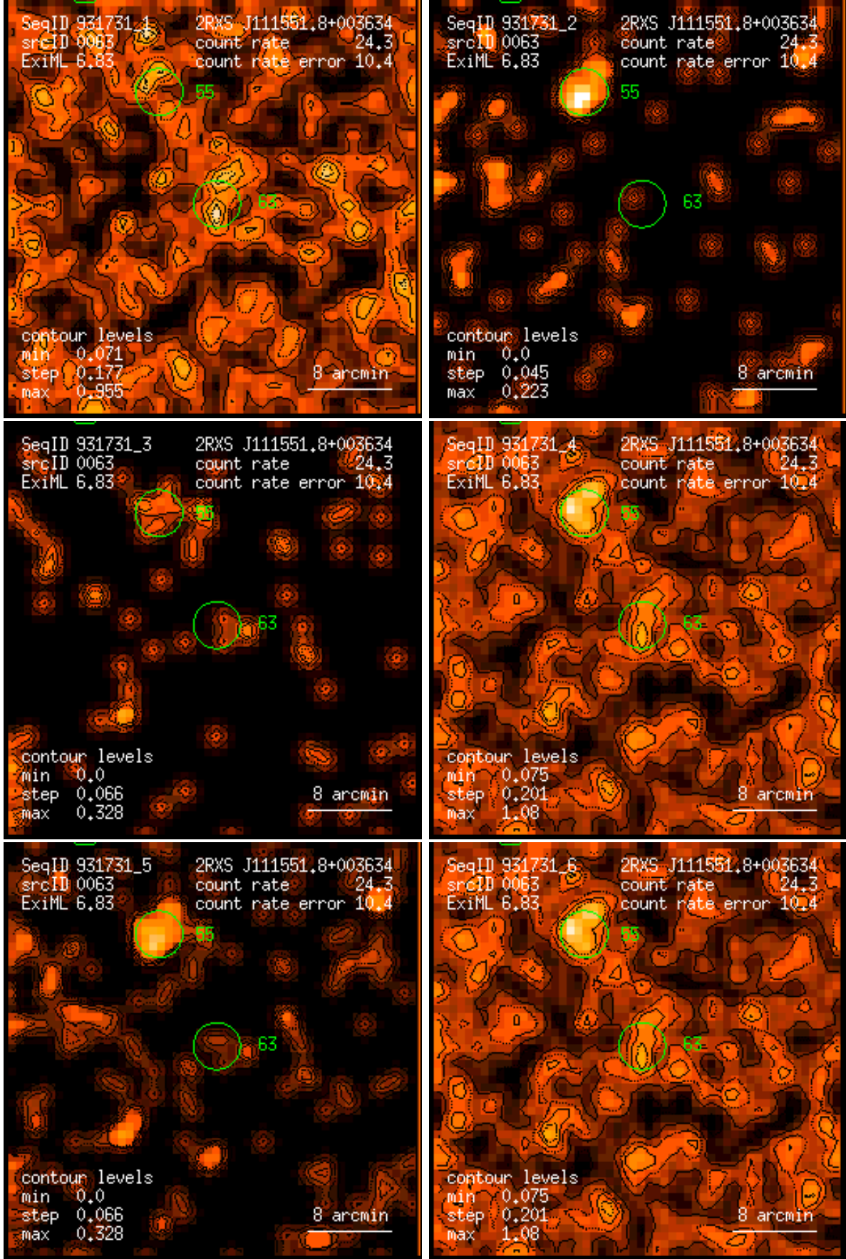
Figure 63: RASS 931731: detection 0063: band rate images, Gaussian filter: (1) PSPC channels 11 – 41, (2) 52 – 90, (3) 91 – 201, (4) 11 – 235, (5) 52 – 201, (6) 11 – 201. Broad band rates in counts/ks. Band rate contour levels in counts/ks/arcmin 2 .
