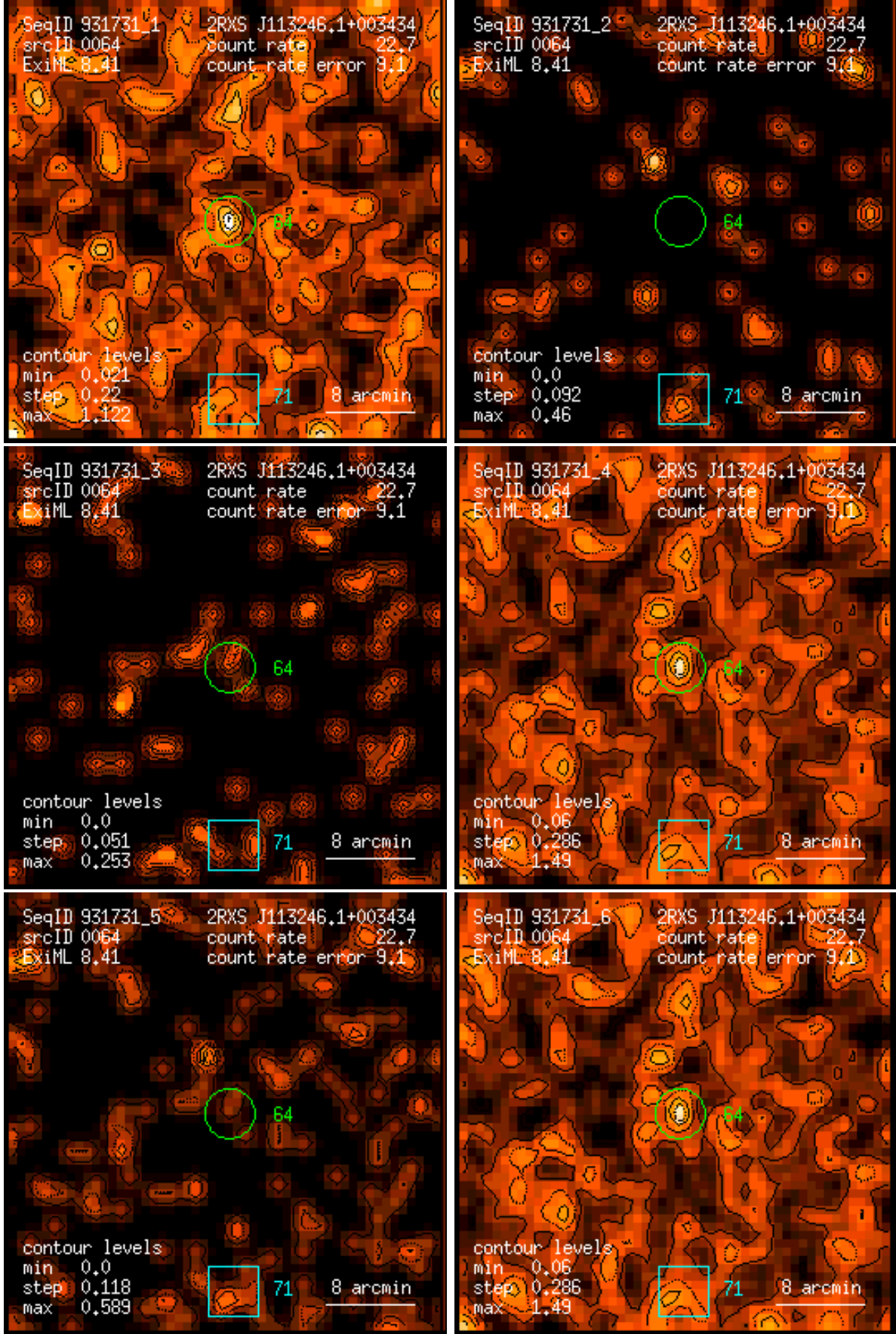
Figure 64: RASS 931731: detection 0064: band rate images, Gaussian filter: (1) PSPC channels 11 – 41, (2) 52 – 90, (3) 91 – 201, (4) 11 – 235, (5) 52 – 201, (6) 11 – 201. Broad band rates in counts/ks. Band rate contour levels in counts/ks/arcmin 2 .
