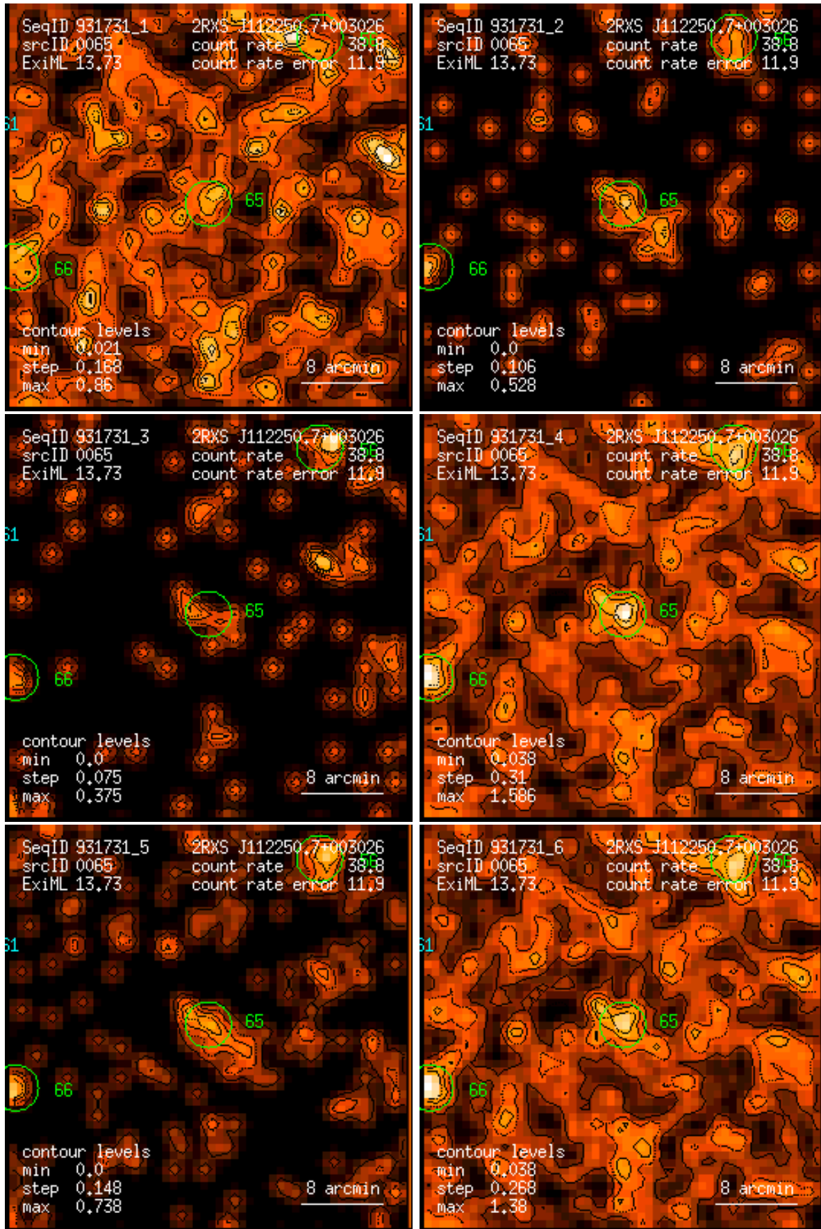
Figure 65: RASS 931731: detection 0065: band rate images, Gaussian filter: (1) PSPC channels 11 – 41, (2) 52 – 90, (3) 91 – 201, (4) 11 – 235, (5) 52 – 201, (6) 11 – 201. Broad band rates in counts/ks. Band rate contour levels in counts/ks/arcmin 2 .
