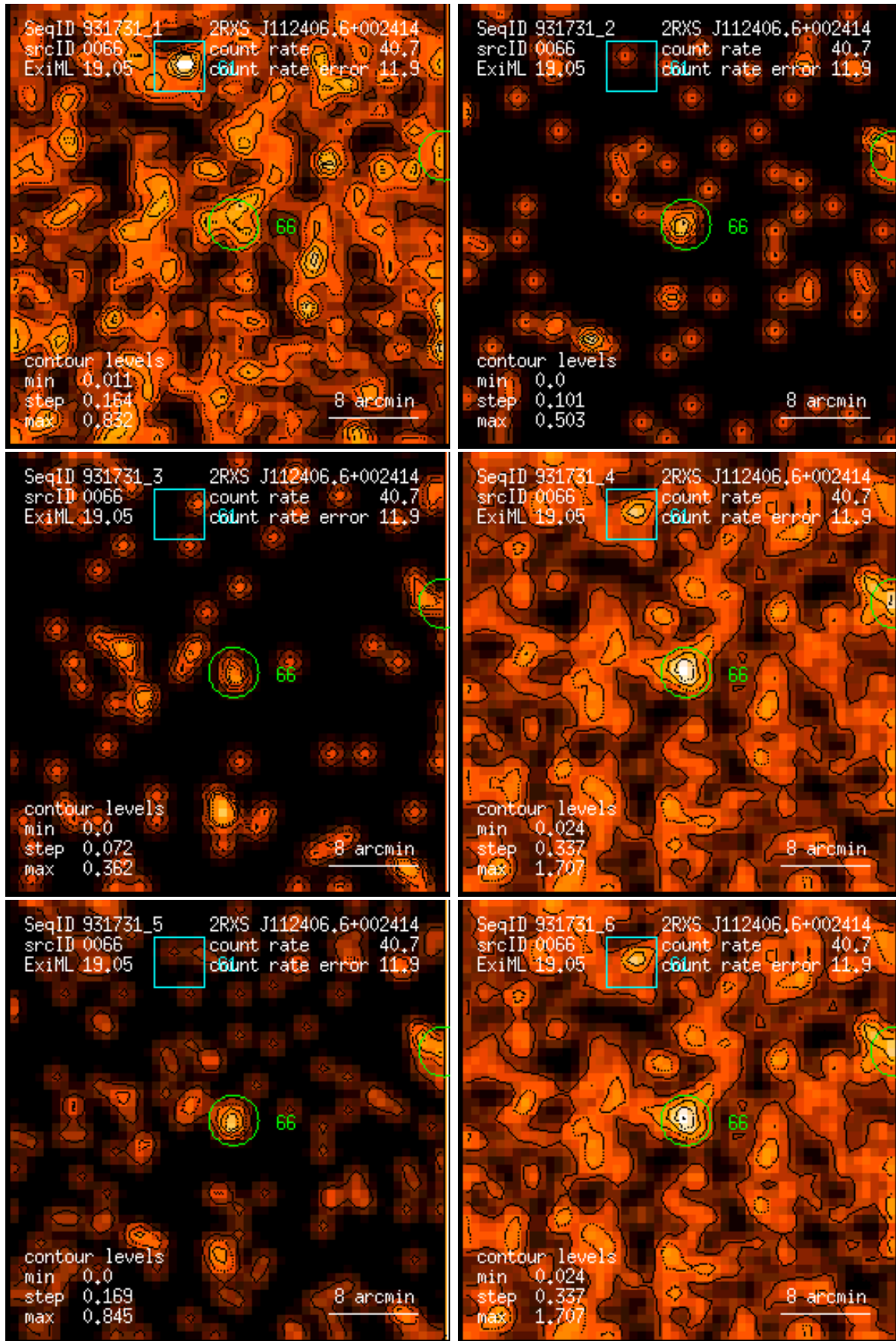
Figure 66: RASS 931731: detection 0066: band rate images, Gaussian filter: (1) PSPC channels 11 – 41, (2) 52 – 90, (3) 91 – 201, (4) 11 – 235, (5) 52 – 201, (6) 11 – 201. Broad band rates in counts/ks. Band rate contour levels in counts/ks/arcmin 2 .
